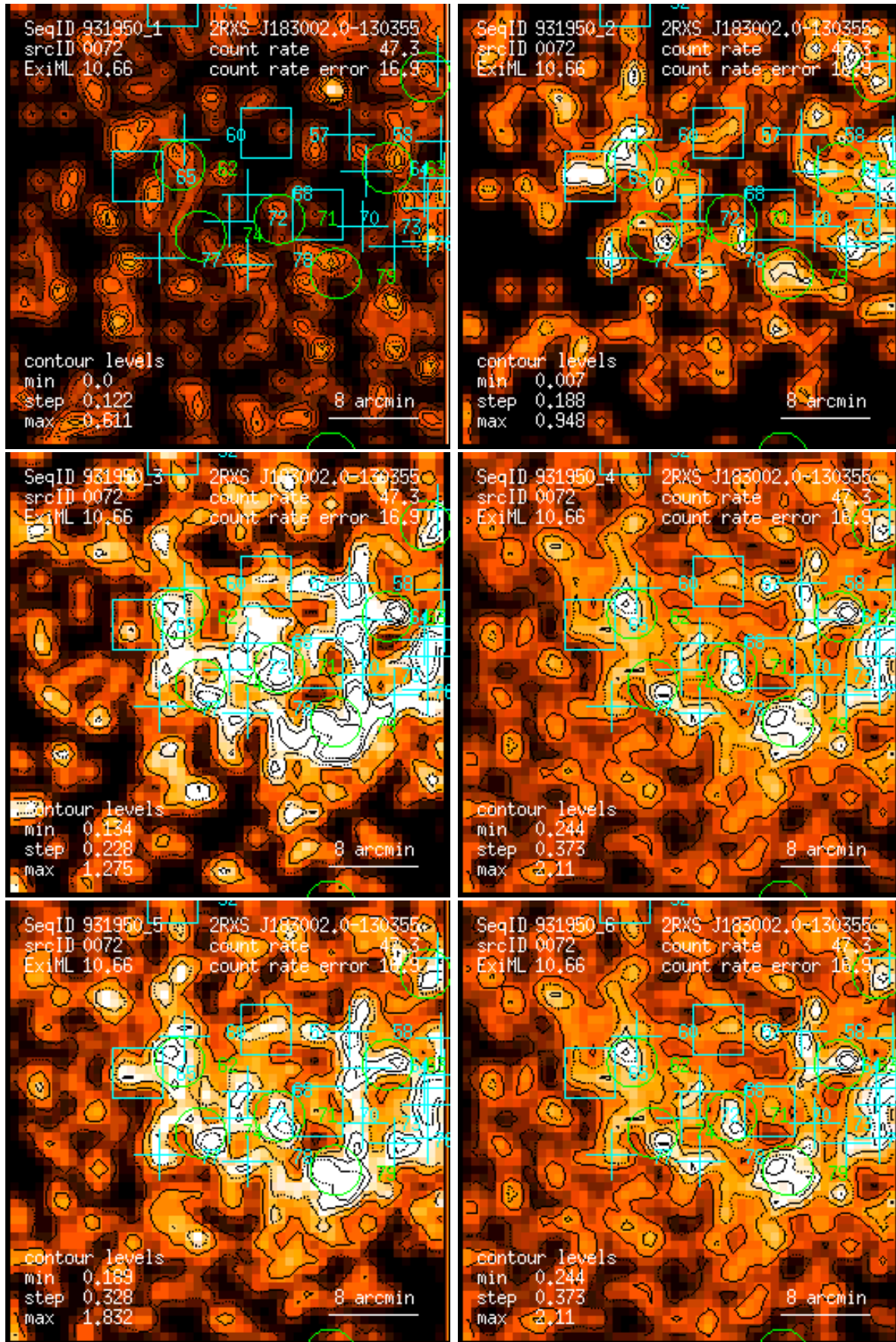
Figure 72: RASS 931950: detection 0072: band rate images, Gaussian filter: (1) PSPC channels 11 – 41, (2) 52 – 90, (3) 91 – 201, (4) 11 – 235, (5) 52 – 201, (6) 11 – 201. Broad band rates in counts/ks. Band rate contour levels in counts/ks/arcmin 2 .
