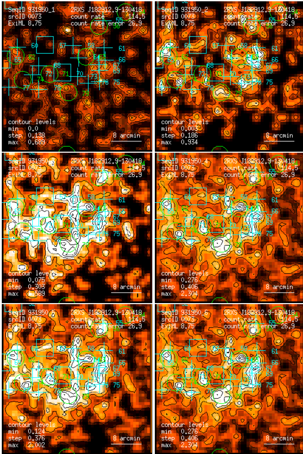
Figure 73: RASS 931950: detection 0073: band rate images, Gaussian filter: (1) PSPC channels 11 – 41, (2) 52 – 90, (3) 91 – 201, (4) 11 – 235, (5) 52 – 201, (6) 11 – 201. Broad band rates in counts/ks. Band rate contour levels in counts/ks/arcmin 2 .
