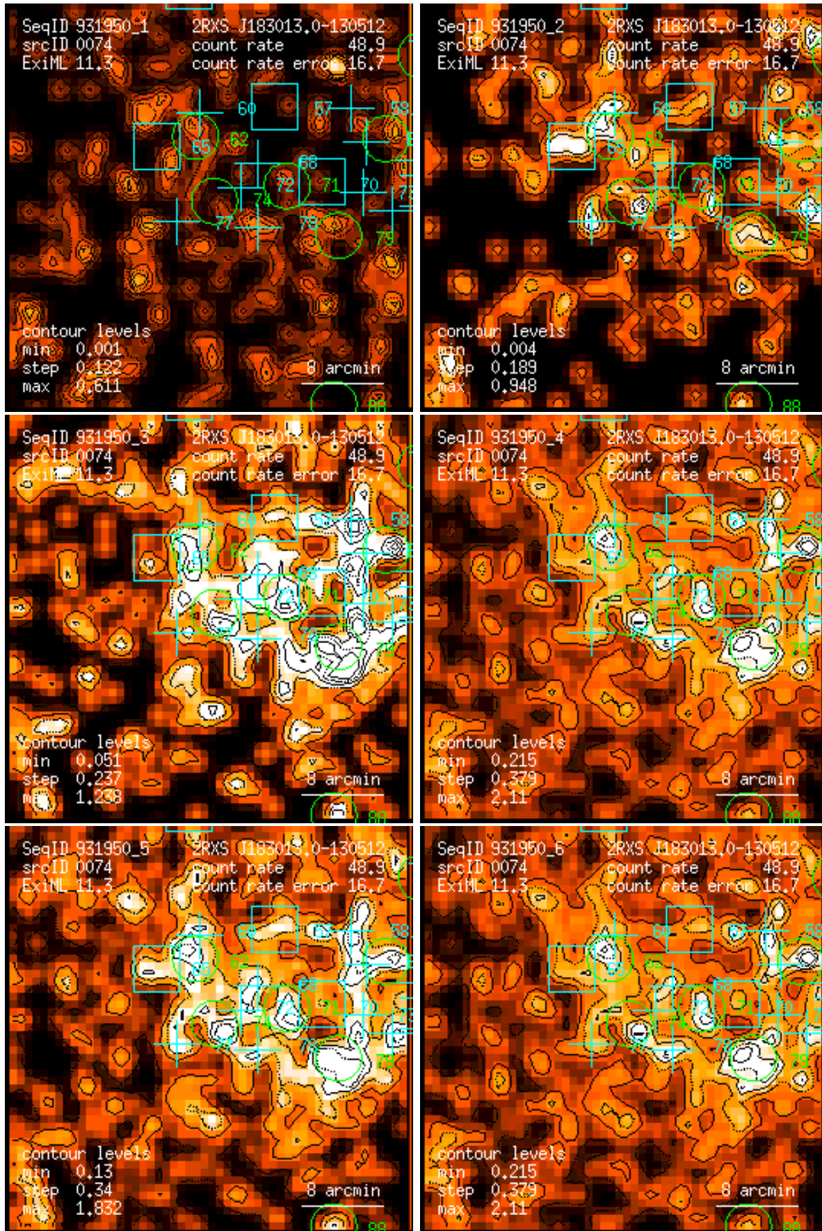
Figure 74: RASS 931950: detection 0074: band rate images, Gaussian filter: (1) PSPC channels 11 – 41, (2) 52 – 90, (3) 91 – 201, (4) 11 – 235, (5) 52 – 201, (6) 11 – 201. Broad band rates in counts/ks. Band rate contour levels in counts/ks/arcmin 2 .
