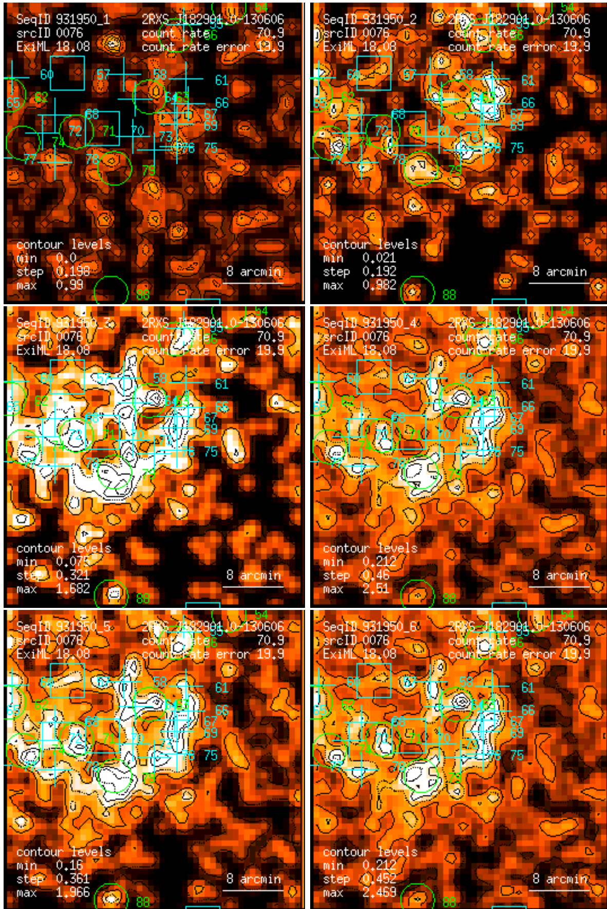
Figure 76: RASS 931950: detection 0076: band rate images, Gaussian filter: (1) PSPC channels 11 – 41, (2) 52 – 90, (3) 91 – 201, (4) 11 – 235, (5) 52 – 201, (6) 11 – 201. Broad band rates in counts/ks. Band rate contour levels in counts/ks/arcmin 2 .
