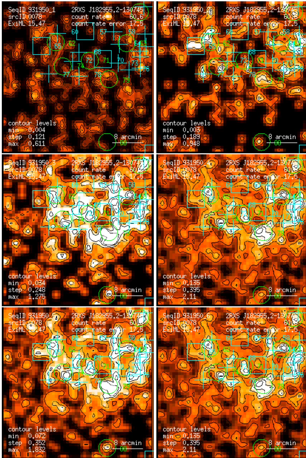
Figure 78: RASS 931950: detection 0078: band rate images, Gaussian filter: (1) PSPC channels 11 – 41, (2) 52 – 90, (3) 91 – 201, (4) 11 – 235, (5) 52 – 201, (6) 11 – 201. Broad band rates in counts/ks. Band rate contour levels in counts/ks/arcmin 2 .
