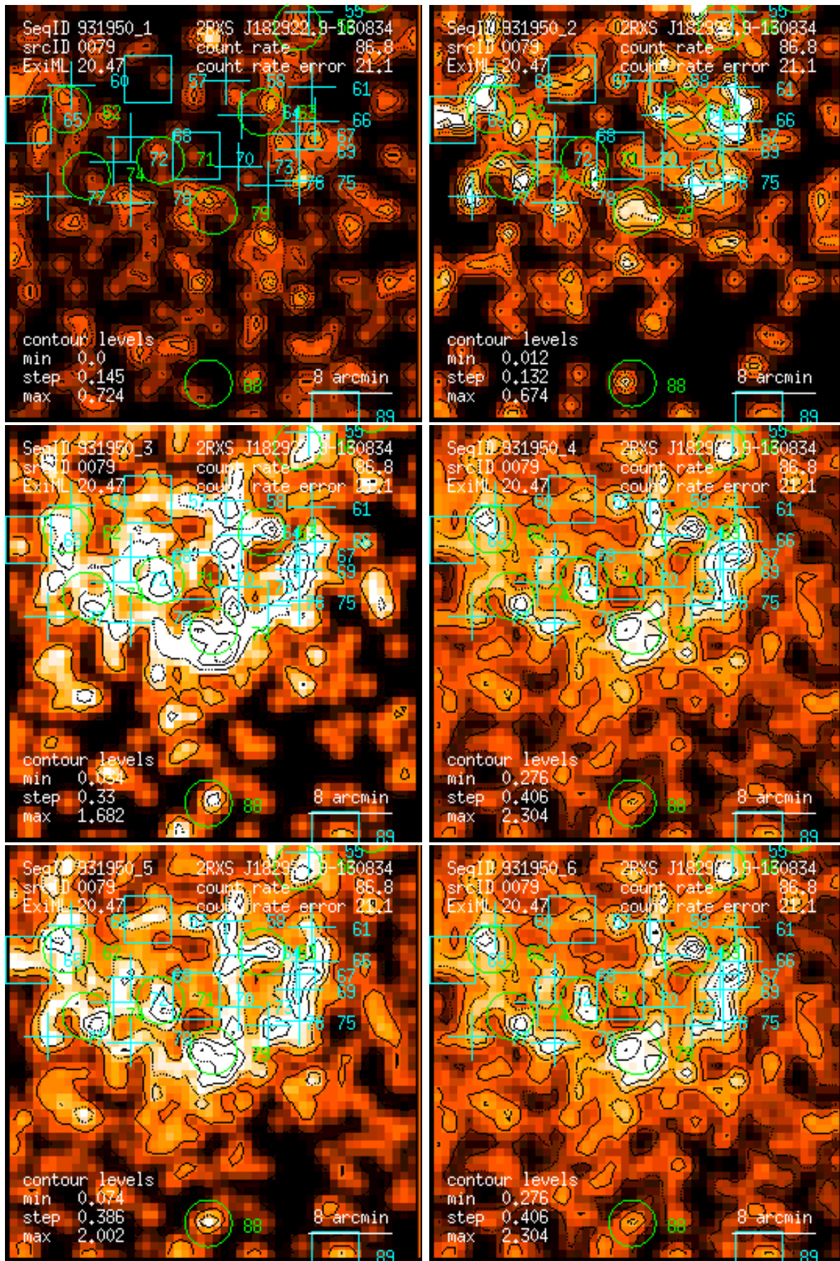
Figure 79: RASS 931950: detection 0079: band rate images, Gaussian filter: (1) PSPC channels 11 – 41, (2) 52 – 90, (3) 91 – 201, (4) 11 – 235, (5) 52 – 201, (6) 11 – 201. Broad band rates in counts/ks. Band rate contour levels in counts/ks/arcmin 2 .
