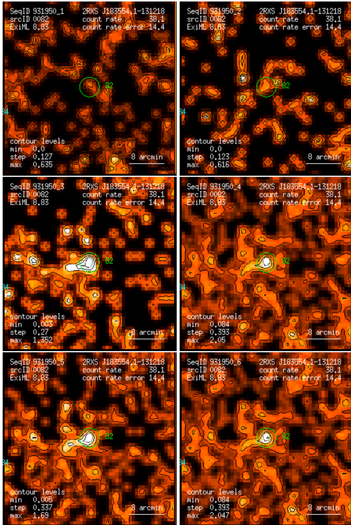
Figure 82: RASS 931950: detection 0082: band rate images, Gaussian filter: (1) PSPC channels 11 – 41, (2) 52 – 90, (3) 91 – 201, (4) 11 – 235, (5) 52 – 201, (6) 11 – 201. Broad band rates in counts/ks. Band rate contour levels in counts/ks/arcmin 2 .
