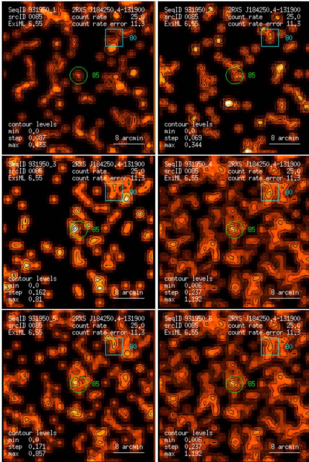
Figure 85: RASS 931950: detection 0085: band rate images, Gaussian filter: (1) PSPC channels 11 – 41, (2) 52 – 90, (3) 91 – 201, (4) 11 – 235, (5) 52 – 201, (6) 11 – 201. Broad band rates in counts/ks. Band rate contour levels in counts/ks/arcmin 2 .
