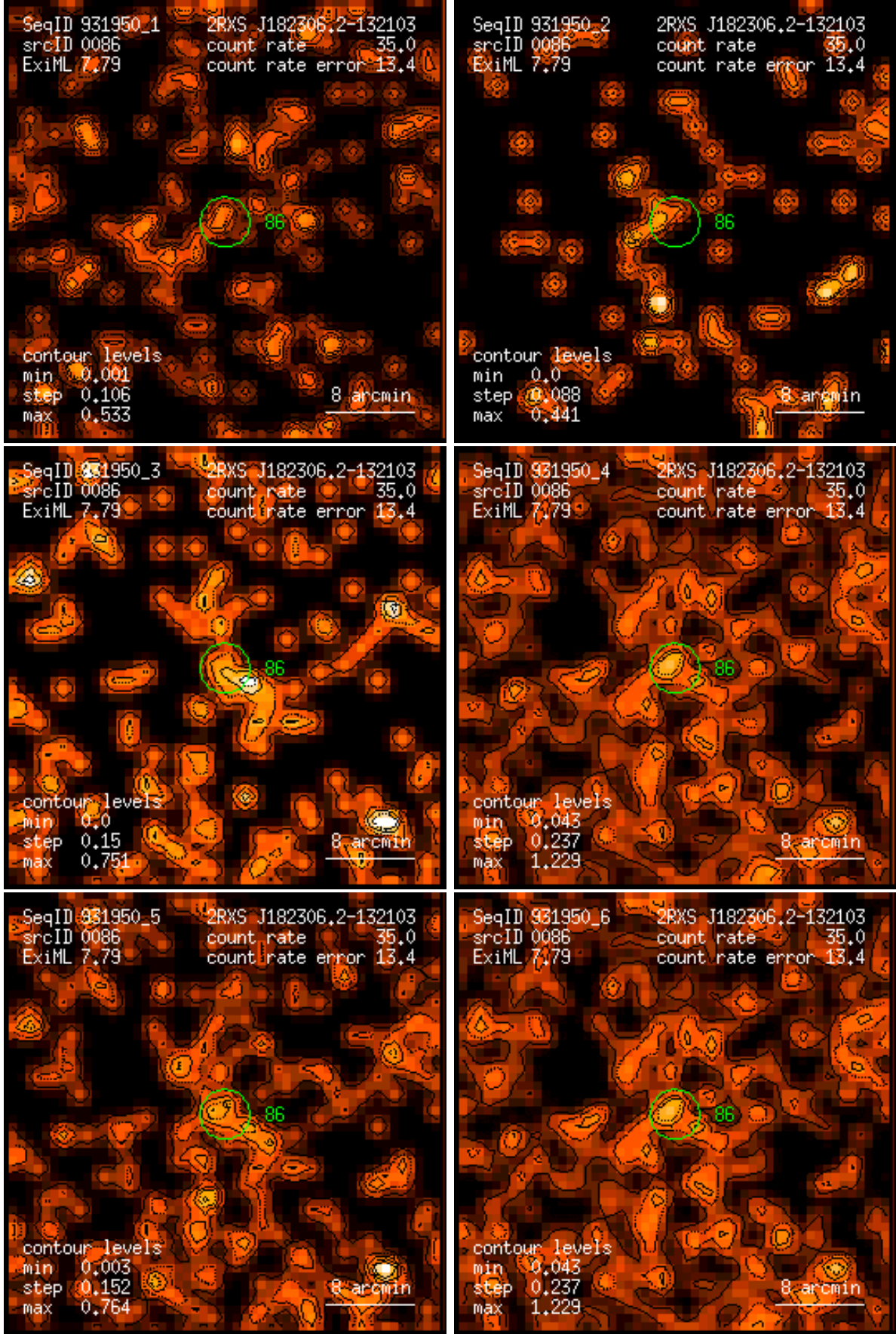
Figure 86: RASS 931950: detection 0086: band rate images, Gaussian filter: (1) PSPC channels 11 – 41, (2) 52 – 90, (3) 91 – 201, (4) 11 – 235, (5) 52 – 201, (6) 11 – 201. Broad band rates in counts/ks. Band rate contour levels in counts/ks/arcmin 2 .
