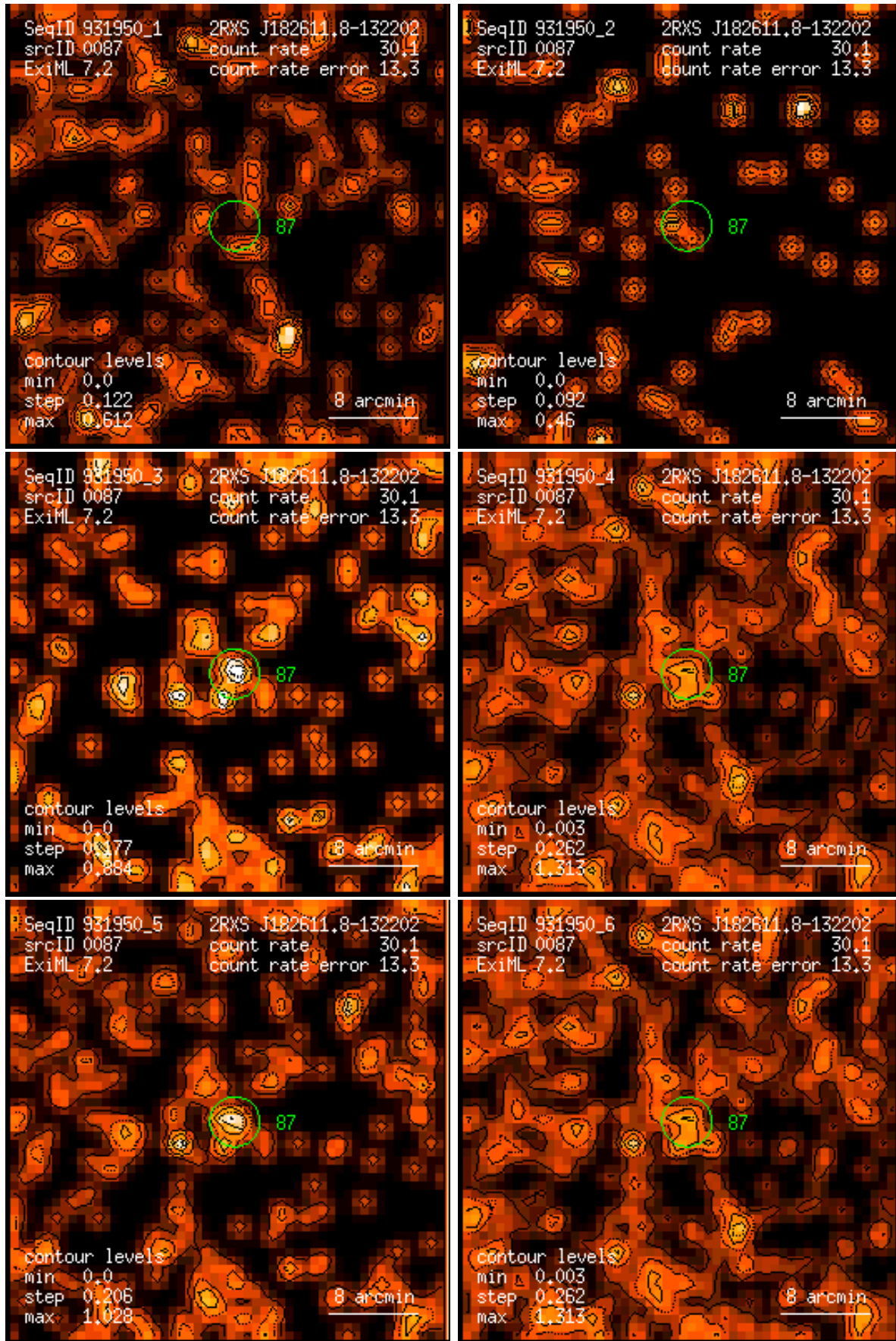
Figure 87: RASS 931950: detection 0087: band rate images, Gaussian filter: (1) PSPC channels 11 – 41, (2) 52 – 90, (3) 91 – 201, (4) 11 – 235, (5) 52 – 201, (6) 11 – 201. Broad band rates in counts/ks. Band rate contour levels in counts/ks/arcmin 2 .
