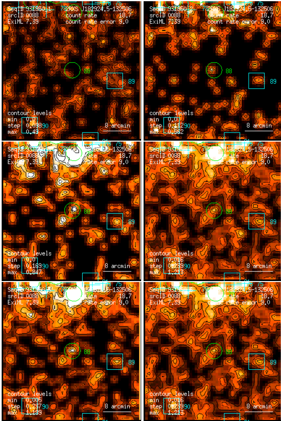
Figure 88: RASS 931950: detection 0088: band rate images, Gaussian filter: (1) PSPC channels 11 – 41, (2) 52 – 90, (3) 91 – 201, (4) 11 – 235, (5) 52 – 201, (6) 11 – 201. Broad band rates in counts/ks. Band rate contour levels in counts/ks/arcmin 2 .
