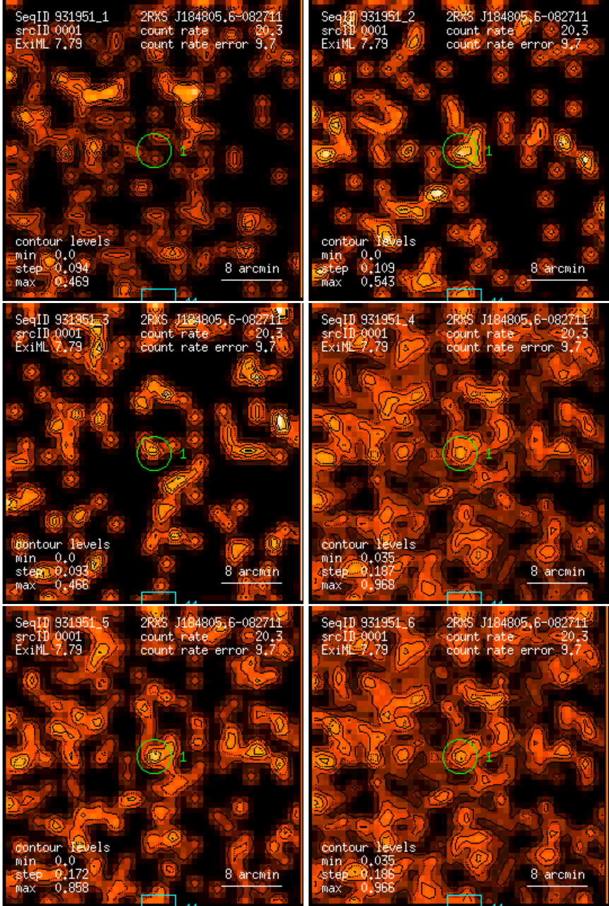
Figure 1: RASS 931951: detection 0001: band rate images, Gaussian filter: (1) PSPC channels 11 – 41, (2) 52 – 90, (3) 91 – 201, (4) 11 – 235, (5) 52 – 201, (6) 11 – 201. Broad band rates in counts/ks. Band rate contour levels in counts/ks/arcmin 2 .
