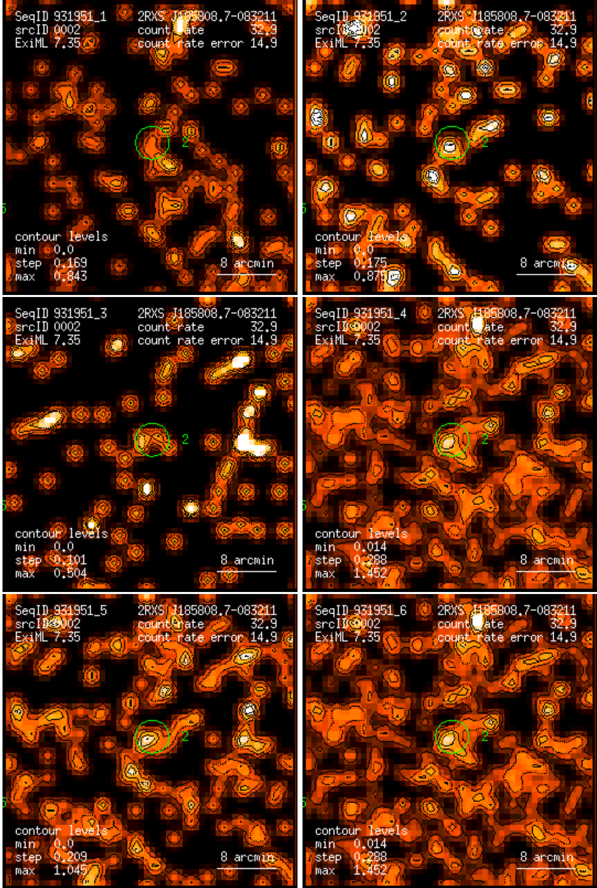
Figure 2: RASS 931951: detection 0002: band rate images, Gaussian filter: (1) PSPC channels 11 – 41, (2) 52 – 90, (3) 91 – 201, (4) 11 – 235, (5) 52 – 201, (6) 11 – 201. Broad band rates in counts/ks. Band rate contour levels in counts/ks/arcmin 2 .
