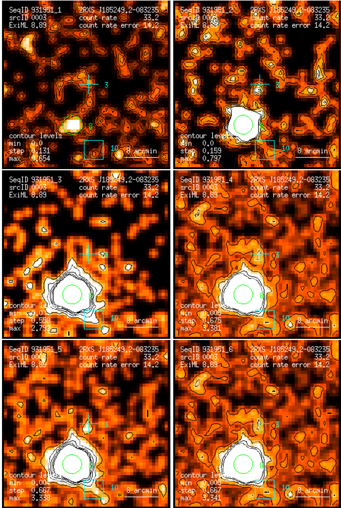
Figure 3: RASS 931951: detection 0003: band rate images, Gaussian filter: (1) PSPC channels 11 – 41, (2) 52 – 90, (3) 91 – 201, (4) 11 – 235, (5) 52 – 201, (6) 11 – 201. Broad band rates in counts/ks. Band rate contour levels in counts/ks/arcmin 2 .
