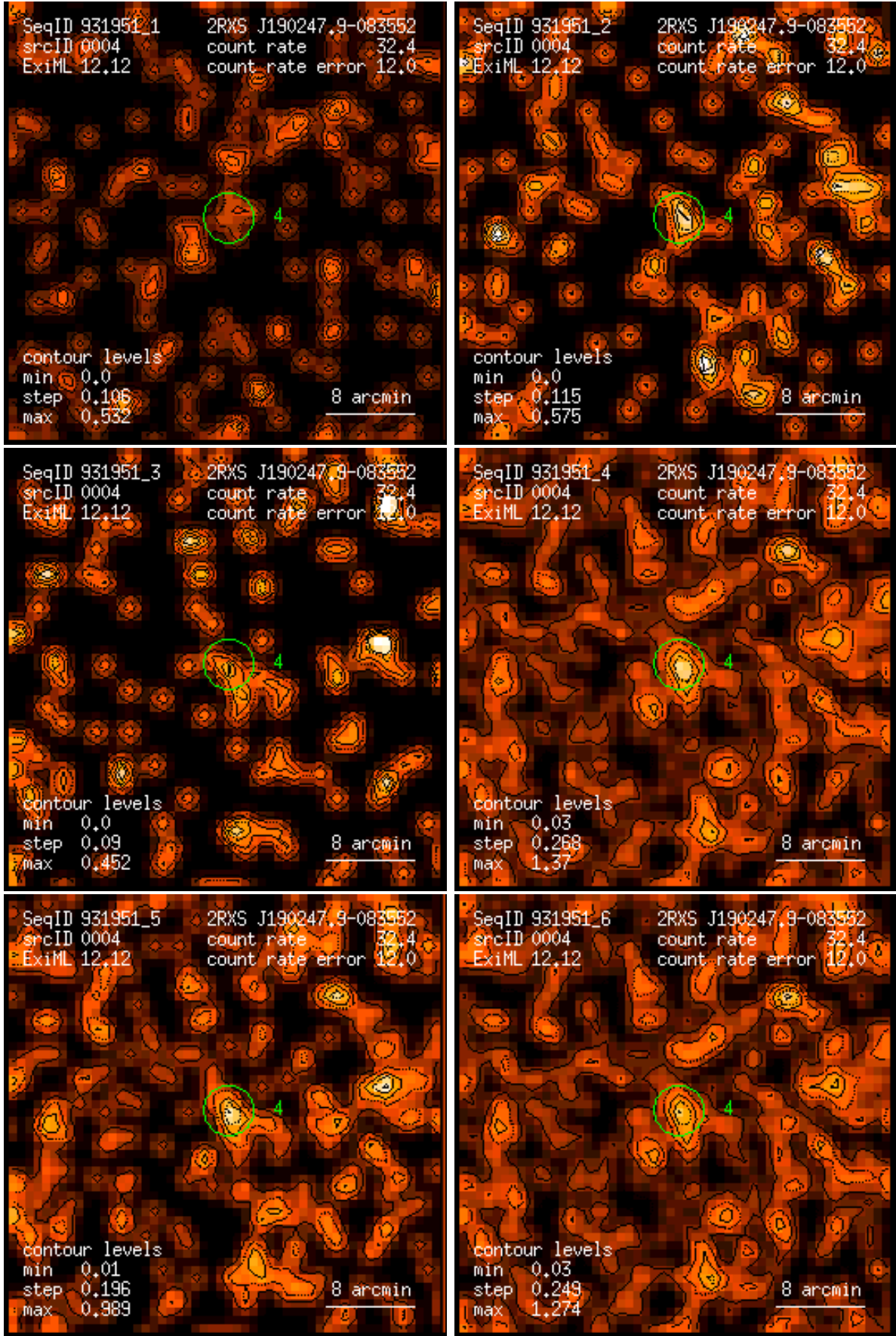
Figure 4: RASS 931951: detection 0004: band rate images, Gaussian filter: (1) PSPC channels 11 – 41, (2) 52 – 90, (3) 91 – 201, (4) 11 – 235, (5) 52 – 201, (6) 11 – 201. Broad band rates in counts/ks. Band rate contour levels in counts/ks/arcmin 2 .
