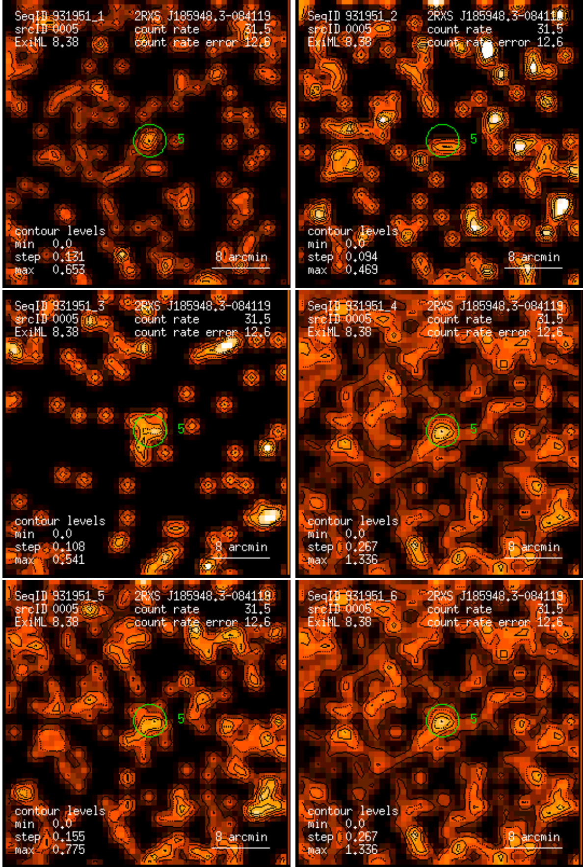
Figure 5: RASS 931951: detection 0005: band rate images, Gaussian filter: (1) PSPC channels 11 – 41, (2) 52 – 90, (3) 91 – 201, (4) 11 – 235, (5) 52 – 201, (6) 11 – 201. Broad band rates in counts/ks. Band rate contour levels in counts/ks/arcmin 2 .
