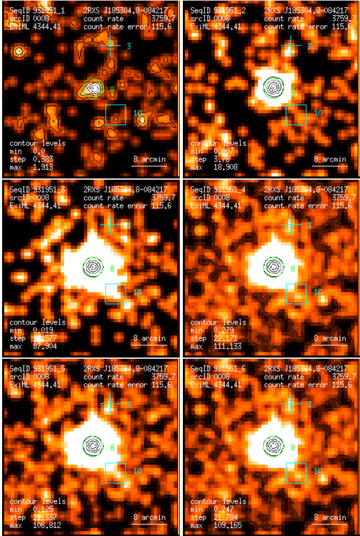
Figure 8: RASS 931951: detection 0008: band rate images, Gaussian filter: (1) PSPC channels 11 – 41, (2) 52 – 90, (3) 91 – 201, (4) 11 – 235, (5) 52 – 201, (6) 11 – 201. Broad band rates in counts/ks. Band rate contour levels in counts/ks/arcmin 2 .
