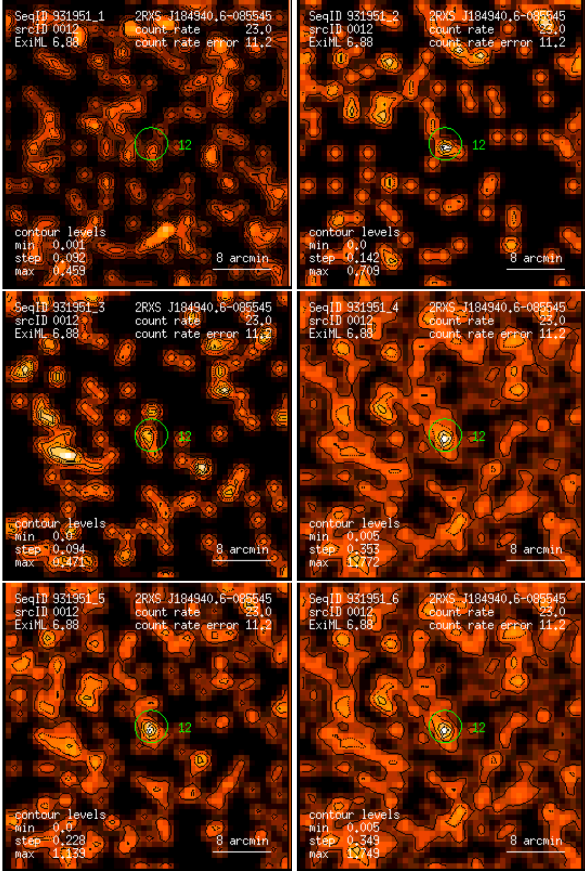
Figure 12: RASS 931951: detection 0012: band rate images, Gaussian filter: (1) PSPC channels 11 – 41, (2) 52 – 90, (3) 91 – 201, (4) 11 – 235, (5) 52 – 201, (6) 11 – 201. Broad band rates in counts/ks. Band rate contour levels in counts/ks/arcmin 2 .
