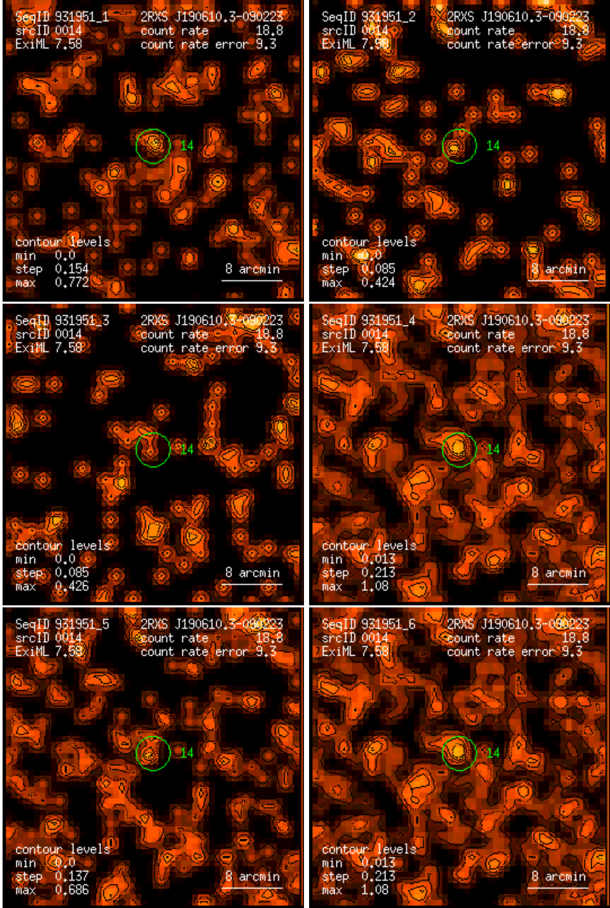
Figure 14: RASS 931951: detection 0014: band rate images, Gaussian filter: (1) PSPC channels 11 – 41, (2) 52 – 90, (3) 91 – 201, (4) 11 – 235, (5) 52 – 201, (6) 11 – 201. Broad band rates in counts/ks. Band rate contour levels in counts/ks/arcmin 2 .
