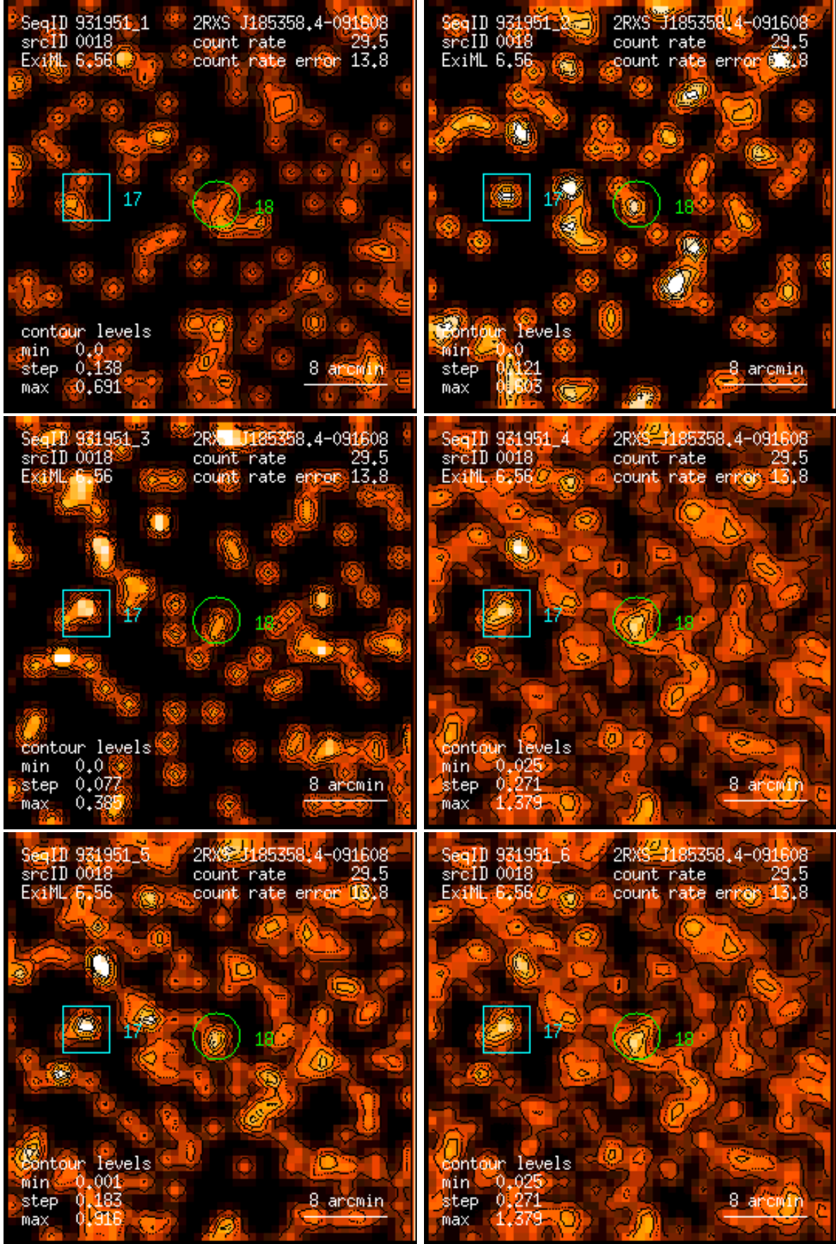
Figure 18: RASS 931951: detection 0018: band rate images, Gaussian filter: (1) PSPC channels 11 – 41, (2) 52 – 90, (3) 91 – 201, (4) 11 – 235, (5) 52 – 201, (6) 11 – 201. Broad band rates in counts/ks. Band rate contour levels in counts/ks/arcmin 2 .
