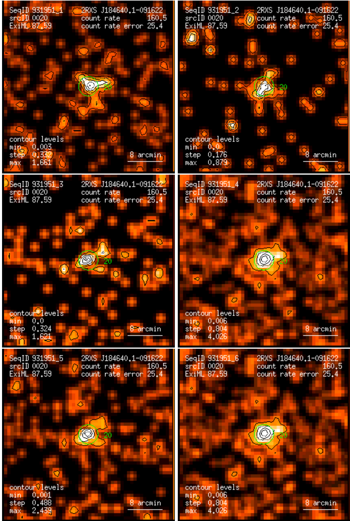
Figure 20: RASS 931951: detection 0020: band rate images, Gaussian filter: (1) PSPC channels 11 – 41, (2) 52 – 90, (3) 91 – 201, (4) 11 – 235, (5) 52 – 201, (6) 11 – 201. Broad band rates in counts/ks. Band rate contour levels in counts/ks/arcmin 2 .
