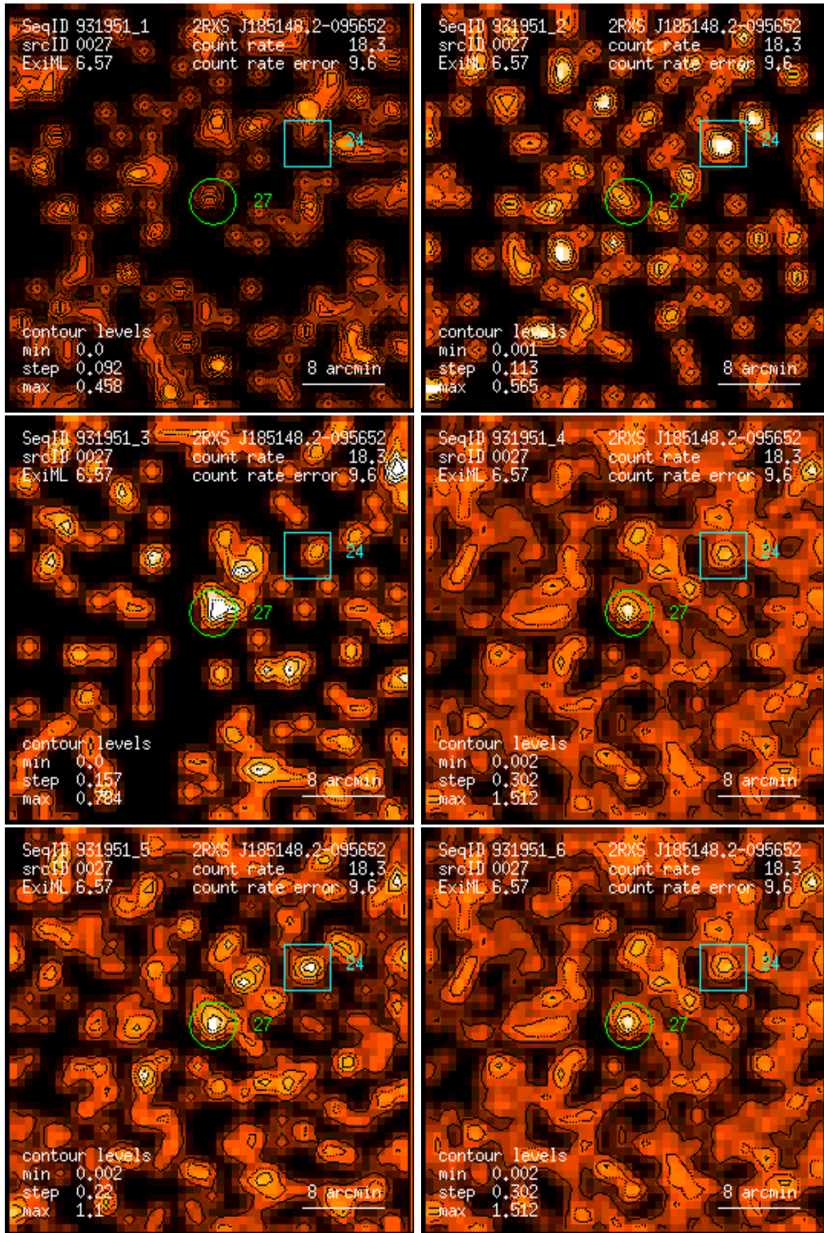
Figure 27: RASS 931951: detection 0027: band rate images, Gaussian filter: (1) PSPC channels 11 – 41, (2) 52 – 90, (3) 91 – 201, (4) 11 – 235, (5) 52 – 201, (6) 11 – 201. Broad band rates in counts/ks. Band rate contour levels in counts/ks/arcmin 2 .
