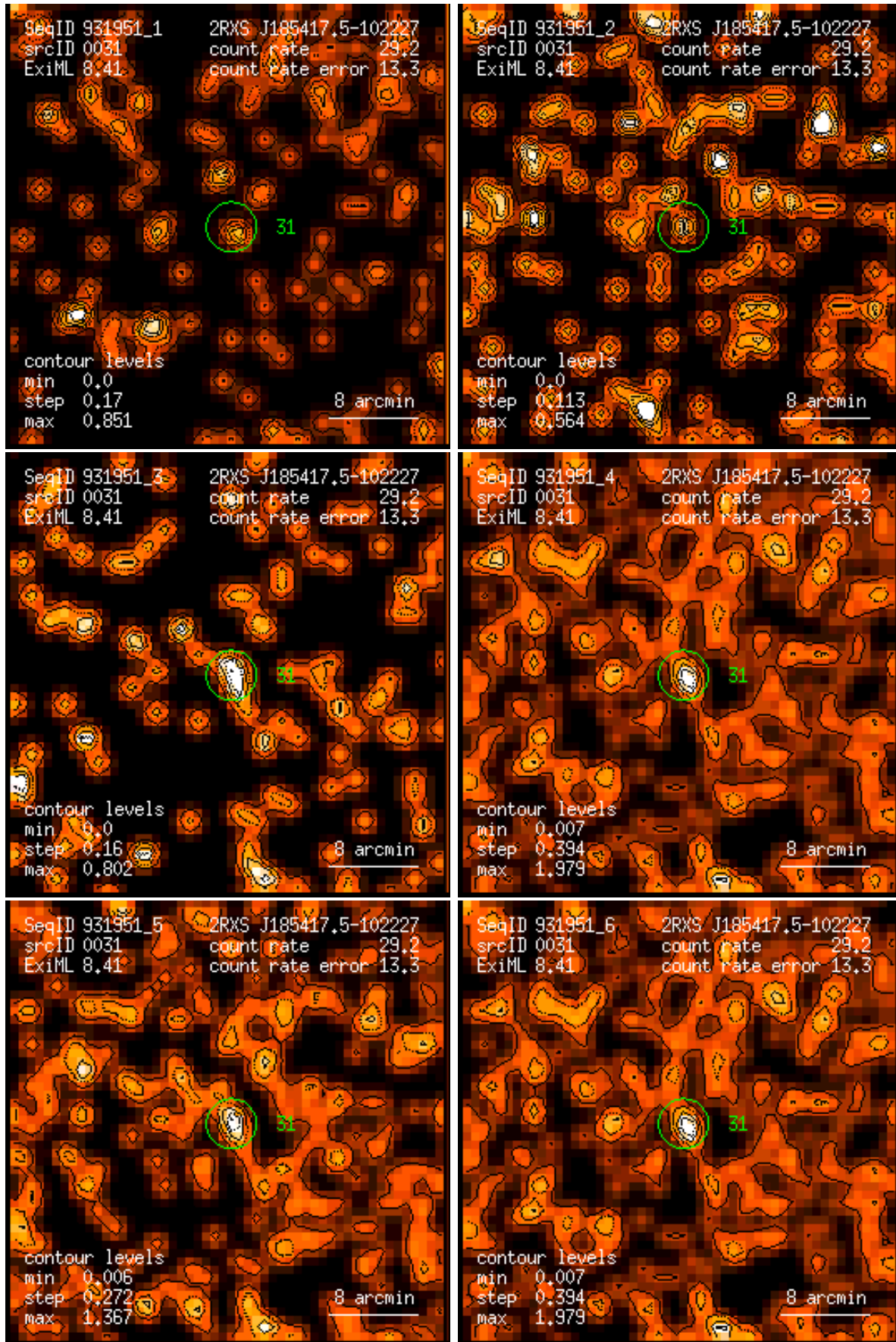
Figure 31: RASS 931951: detection 0031: band rate images, Gaussian filter: (1) PSPC channels 11 – 41, (2) 52 – 90, (3) 91 – 201, (4) 11 – 235, (5) 52 – 201, (6) 11 – 201. Broad band rates in counts/ks. Band rate contour levels in counts/ks/arcmin 2 .
