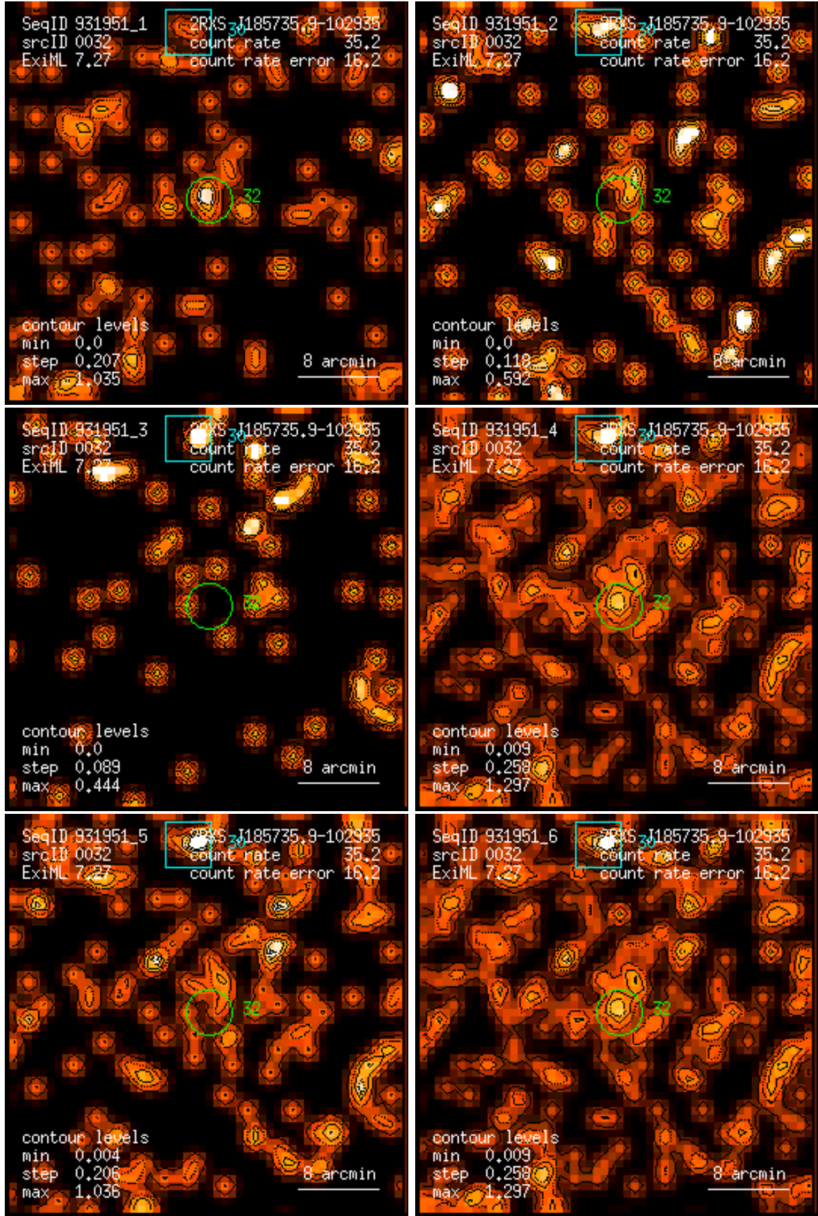
Figure 32: RASS 931951: detection 0032: band rate images, Gaussian filter: (1) PSPC channels 11 – 41, (2) 52 – 90, (3) 91 – 201, (4) 11 – 235, (5) 52 – 201, (6) 11 – 201. Broad band rates in counts/ks. Band rate contour levels in counts/ks/arcmin 2 .
