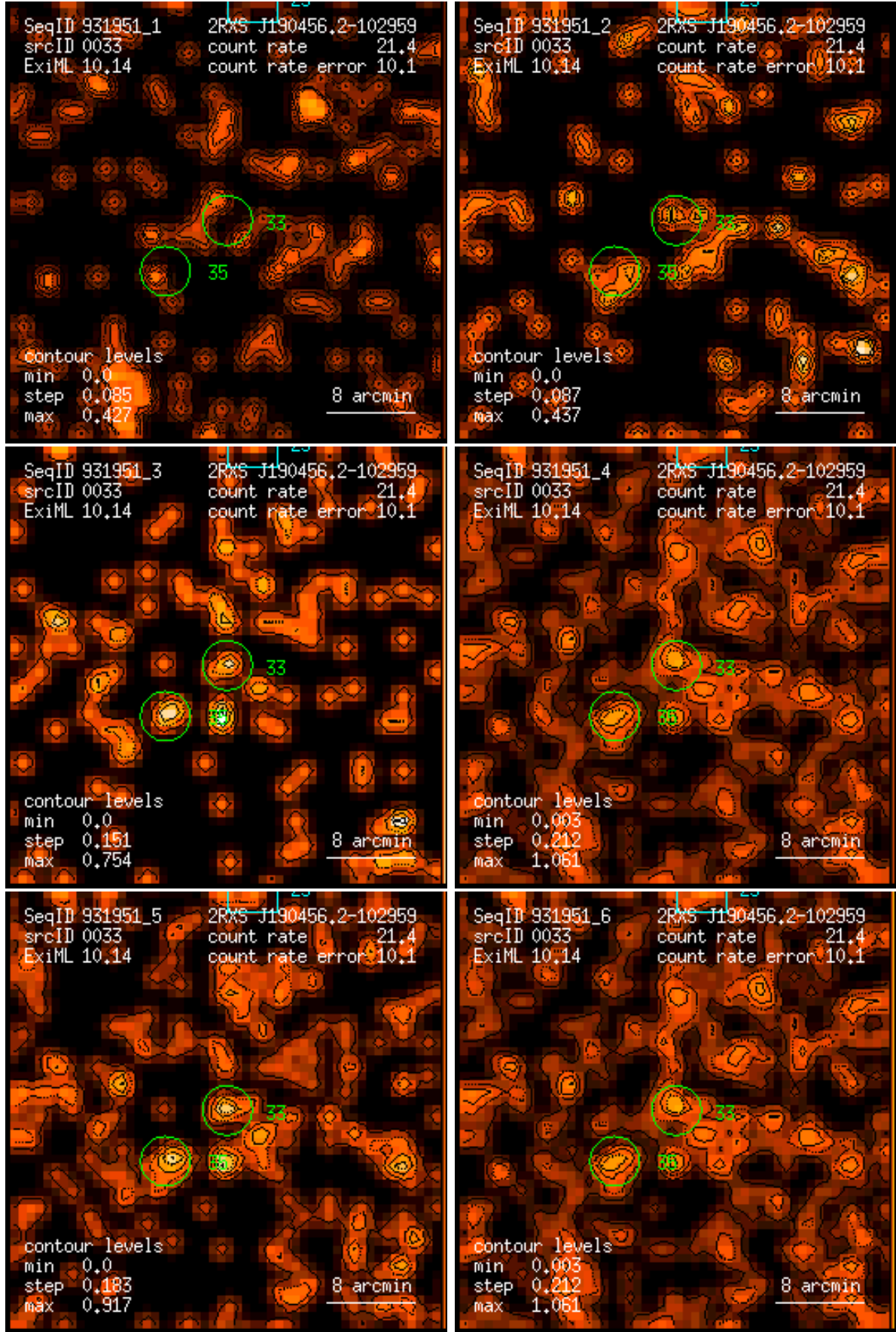
Figure 33: RASS 931951: detection 0033: band rate images, Gaussian filter: (1) PSPC channels 11 – 41, (2) 52 – 90, (3) 91 – 201, (4) 11 – 235, (5) 52 – 201, (6) 11 – 201. Broad band rates in counts/ks. Band rate contour levels in counts/ks/arcmin 2 .
