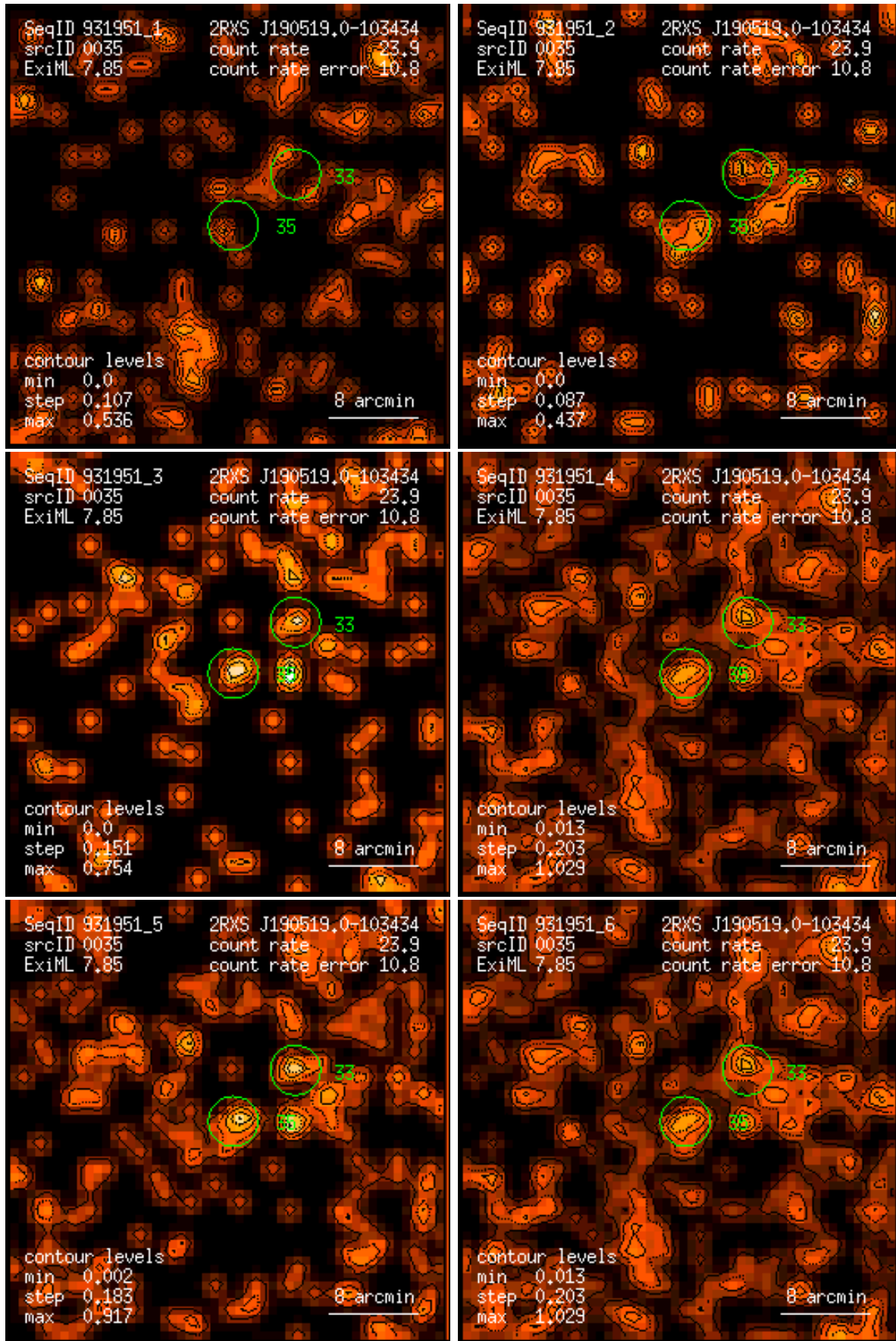
Figure 35: RASS 931951: detection 0035: band rate images, Gaussian filter: (1) PSPC channels 11 – 41, (2) 52 – 90, (3) 91 – 201, (4) 11 – 235, (5) 52 – 201, (6) 11 – 201. Broad band rates in counts/ks. Band rate contour levels in counts/ks/arcmin 2 .
