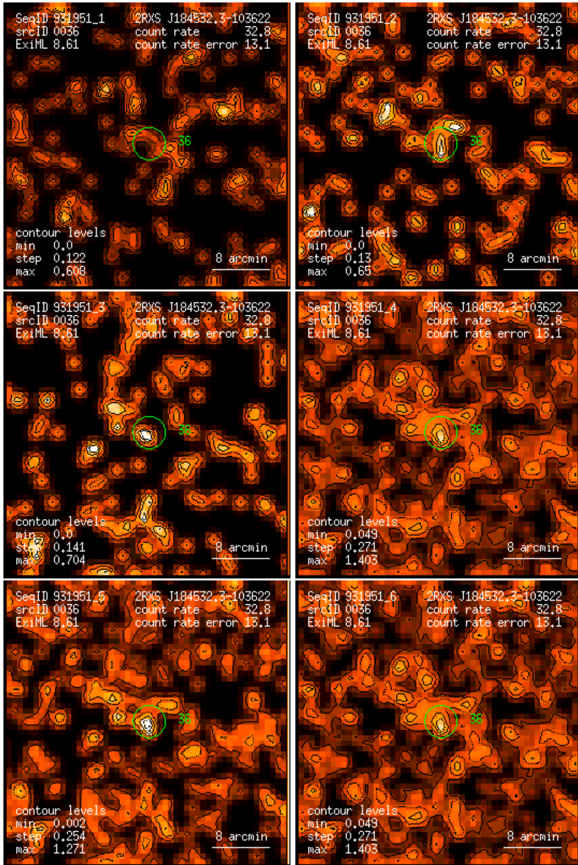
Figure 36: RASS 931951: detection 0036: band rate images, Gaussian filter: (1) PSPC channels 11 – 41, (2) 52 – 90, (3) 91 – 201, (4) 11 – 235, (5) 52 – 201, (6) 11 – 201. Broad band rates in counts/ks. Band rate contour levels in counts/ks/arcmin 2 .
