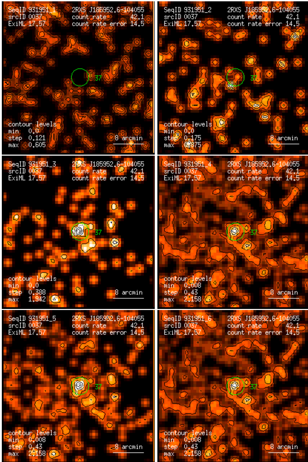
Figure 37: RASS 931951: detection 0037: band rate images, Gaussian filter: (1) PSPC channels 11 – 41, (2) 52 – 90, (3) 91 – 201, (4) 11 – 235, (5) 52 – 201, (6) 11 – 201. Broad band rates in counts/ks. Band rate contour levels in counts/ks/arcmin 2 .
