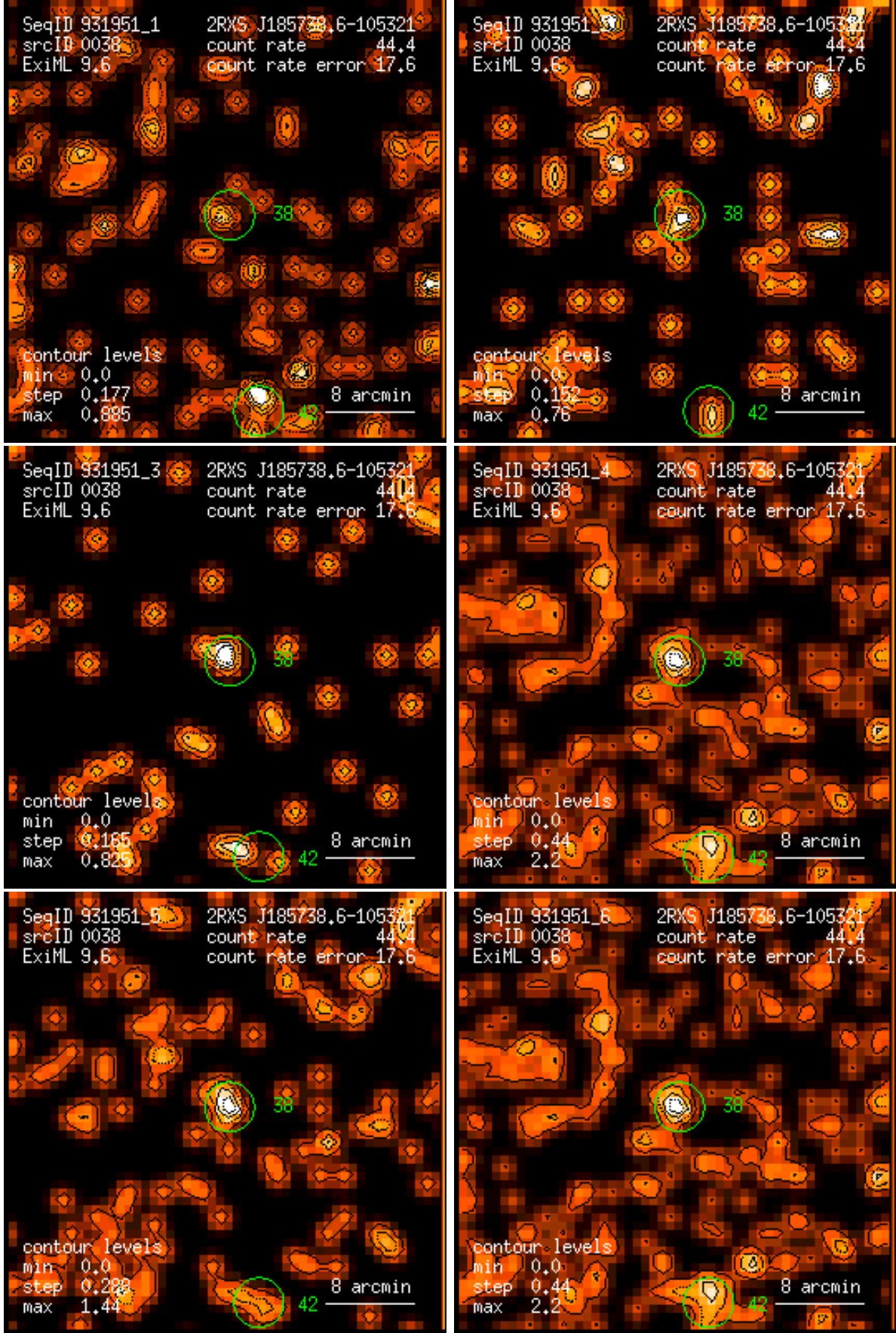
Figure 38: RASS 931951: detection 0038: band rate images, Gaussian filter: (1) PSPC channels 11 – 41, (2) 52 – 90, (3) 91 – 201, (4) 11 – 235, (5) 52 – 201, (6) 11 – 201. Broad band rates in counts/ks. Band rate contour levels in counts/ks/arcmin 2 .
