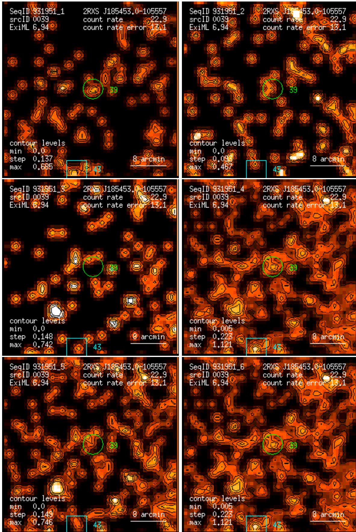
Figure 39: RASS 931951: detection 0039: band rate images, Gaussian filter: (1) PSPC channels 11 – 41, (2) 52 – 90, (3) 91 – 201, (4) 11 – 235, (5) 52 – 201, (6) 11 – 201. Broad band rates in counts/ks. Band rate contour levels in counts/ks/arcmin 2 .
