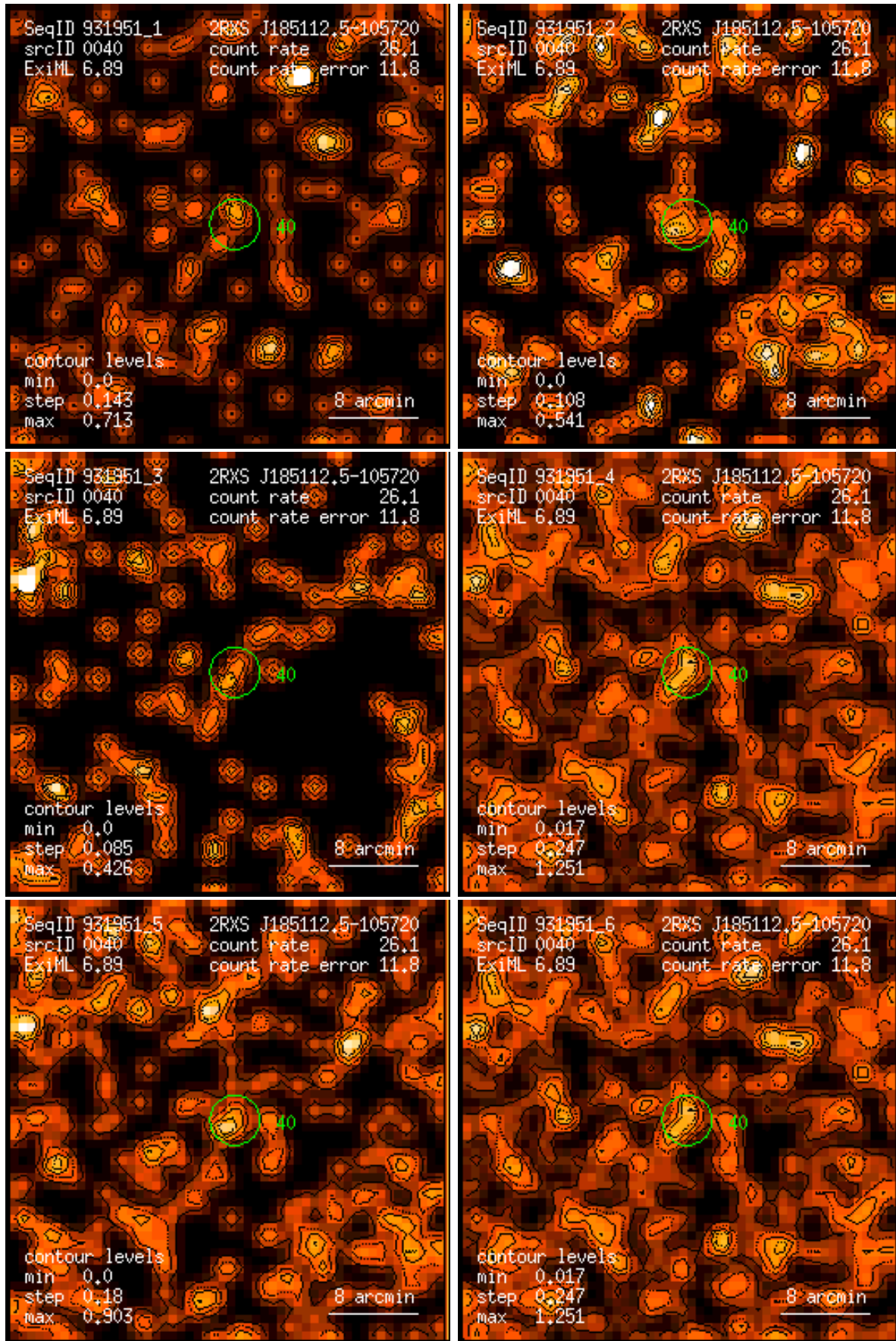
Figure 40: RASS 931951: detection 0040: band rate images, Gaussian filter: (1) PSPC channels 11 – 41, (2) 52 – 90, (3) 91 – 201, (4) 11 – 235, (5) 52 – 201, (6) 11 – 201. Broad band rates in counts/ks. Band rate contour levels in counts/ks/arcmin 2 .
