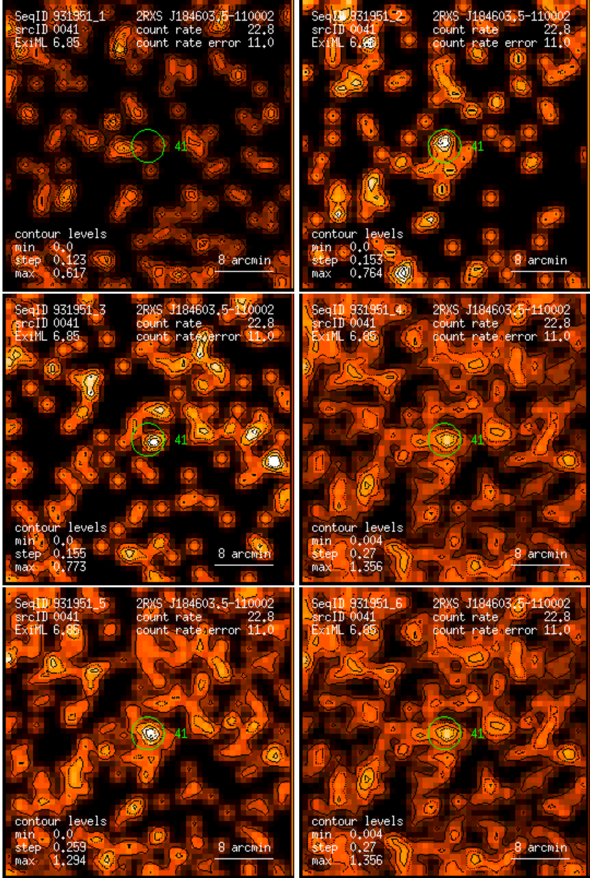
Figure 41: RASS 931951: detection 0041: band rate images, Gaussian filter: (1) PSPC channels 11 – 41, (2) 52 – 90, (3) 91 – 201, (4) 11 – 235, (5) 52 – 201, (6) 11 – 201. Broad band rates in counts/ks. Band rate contour levels in counts/ks/arcmin 2 .
