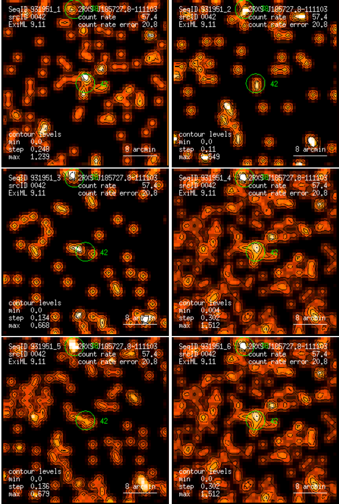
Figure 42: RASS 931951: detection 0042: band rate images, Gaussian filter: (1) PSPC channels 11 – 41, (2) 52 – 90, (3) 91 – 201, (4) 11 – 235, (5) 52 – 201, (6) 11 – 201. Broad band rates in counts/ks. Band rate contour levels in counts/ks/arcmin 2 .
