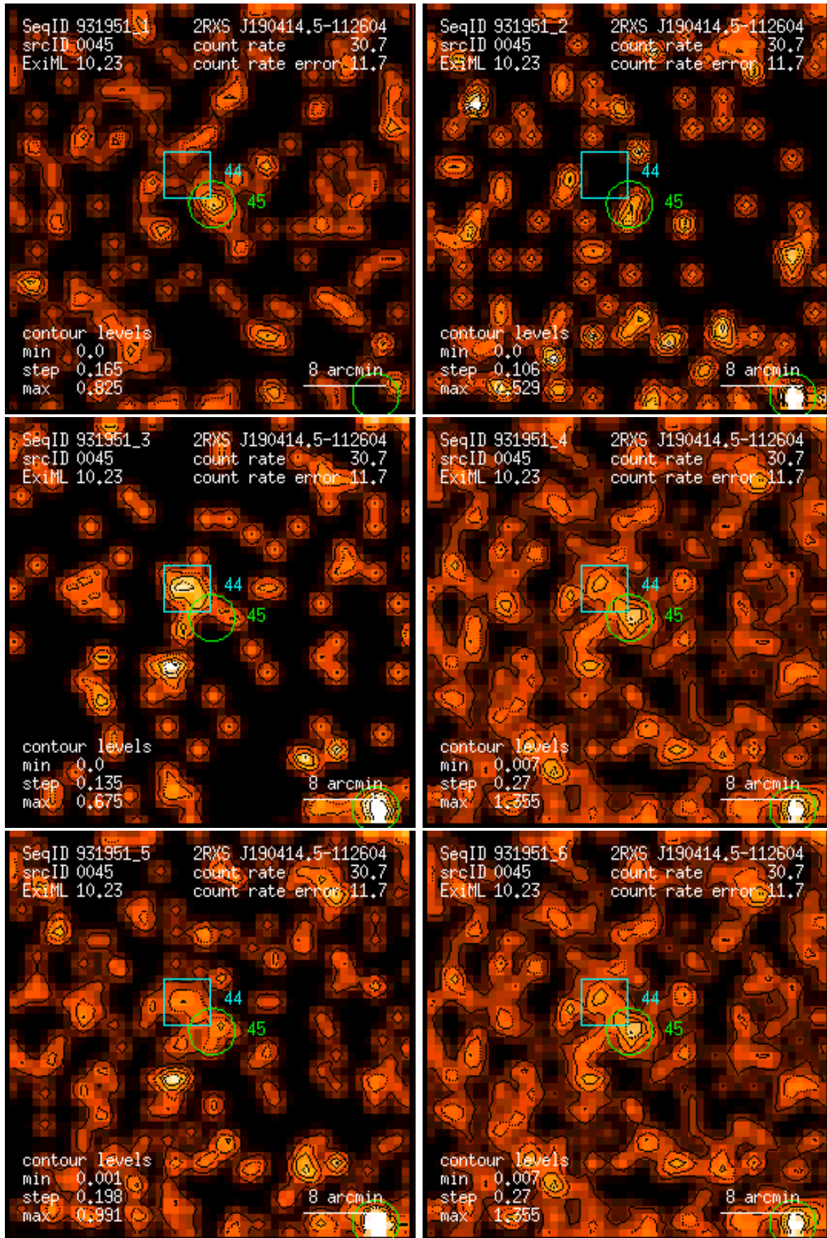
Figure 45: RASS 931951: detection 0045: band rate images, Gaussian filter: (1) PSPC channels 11 – 41, (2) 52 – 90, (3) 91 – 201, (4) 11 – 235, (5) 52 – 201, (6) 11 – 201. Broad band rates in counts/ks. Band rate contour levels in counts/ks/arcmin 2 .
