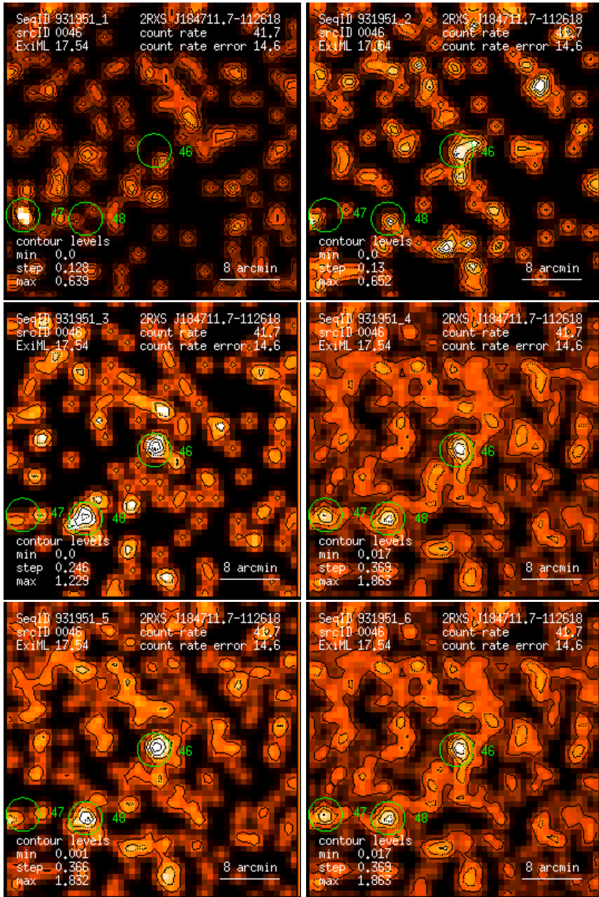
Figure 46: RASS 931951: detection 0046: band rate images, Gaussian filter: (1) PSPC channels 11 – 41, (2) 52 – 90, (3) 91 – 201, (4) 11 – 235, (5) 52 – 201, (6) 11 – 201. Broad band rates in counts/ks. Band rate contour levels in counts/ks/arcmin 2 .
