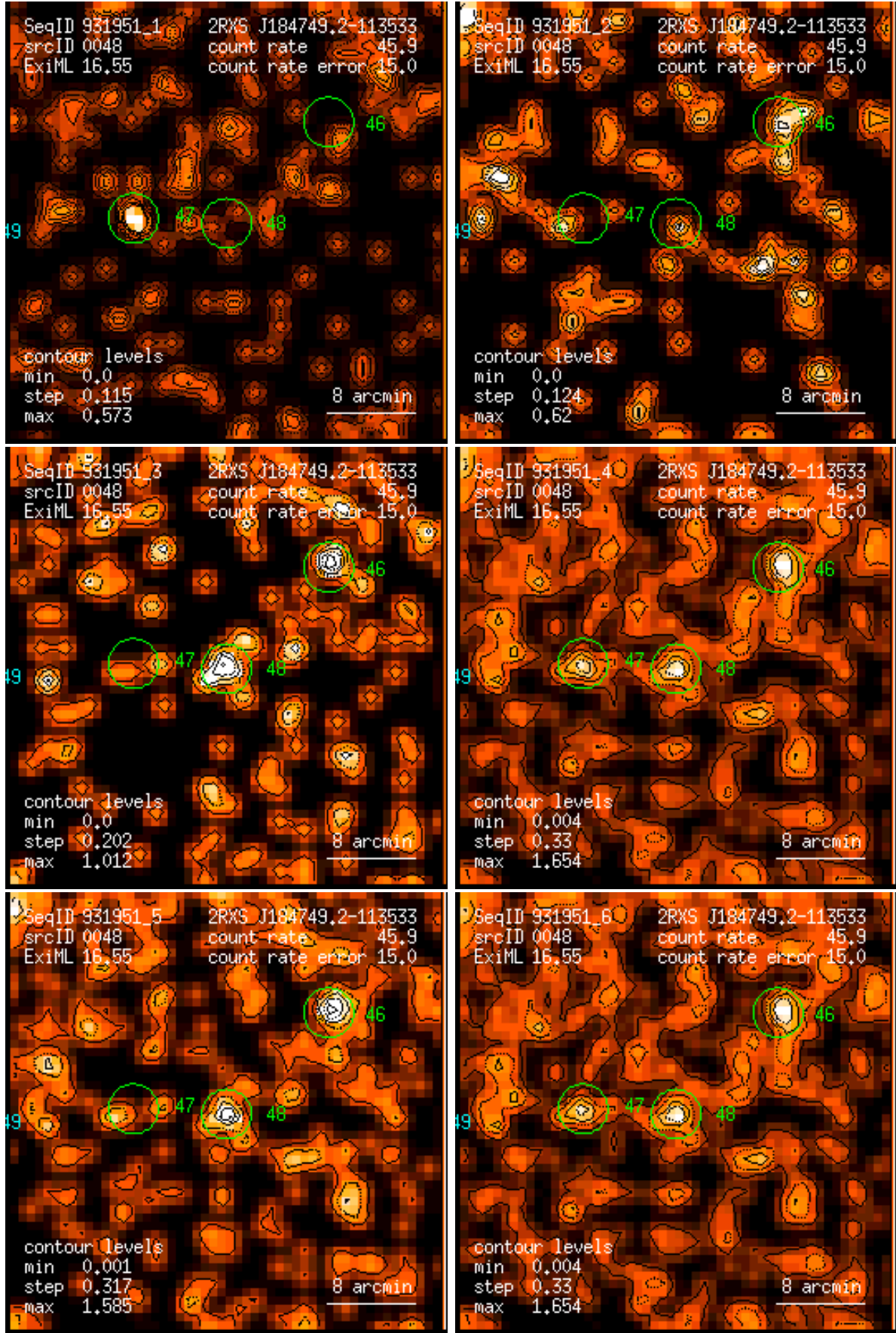
Figure 48: RASS 931951: detection 0048: band rate images, Gaussian filter: (1) PSPC channels 11 – 41, (2) 52 – 90, (3) 91 – 201, (4) 11 – 235, (5) 52 – 201, (6) 11 – 201. Broad band rates in counts/ks. Band rate contour levels in counts/ks/arcmin 2 .
