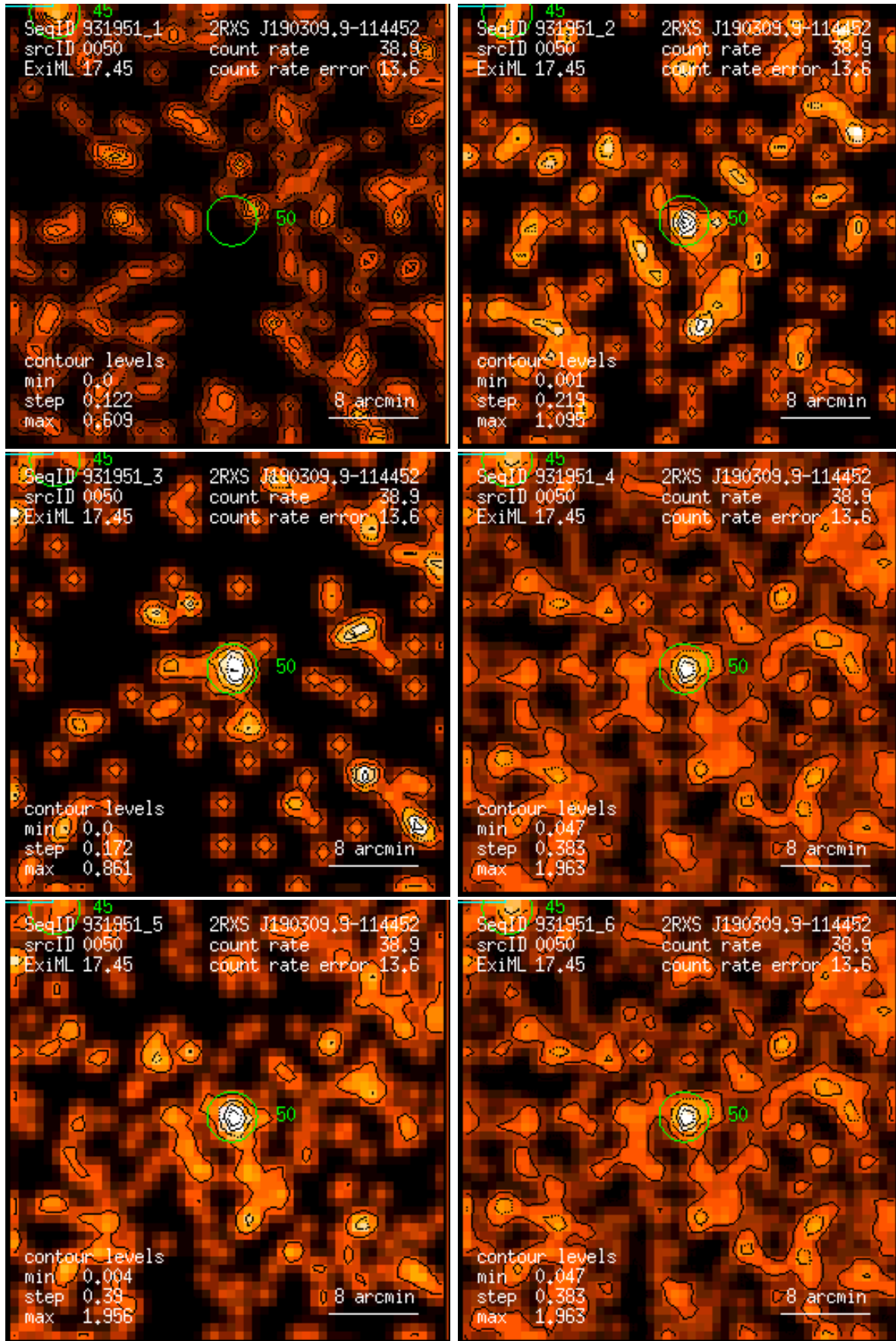
Figure 50: RASS 931951: detection 0050: band rate images, Gaussian filter: (1) PSPC channels 11 – 41, (2) 52 – 90, (3) 91 – 201, (4) 11 – 235, (5) 52 – 201, (6) 11 – 201. Broad band rates in counts/ks. Band rate contour levels in counts/ks/arcmin 2 .
