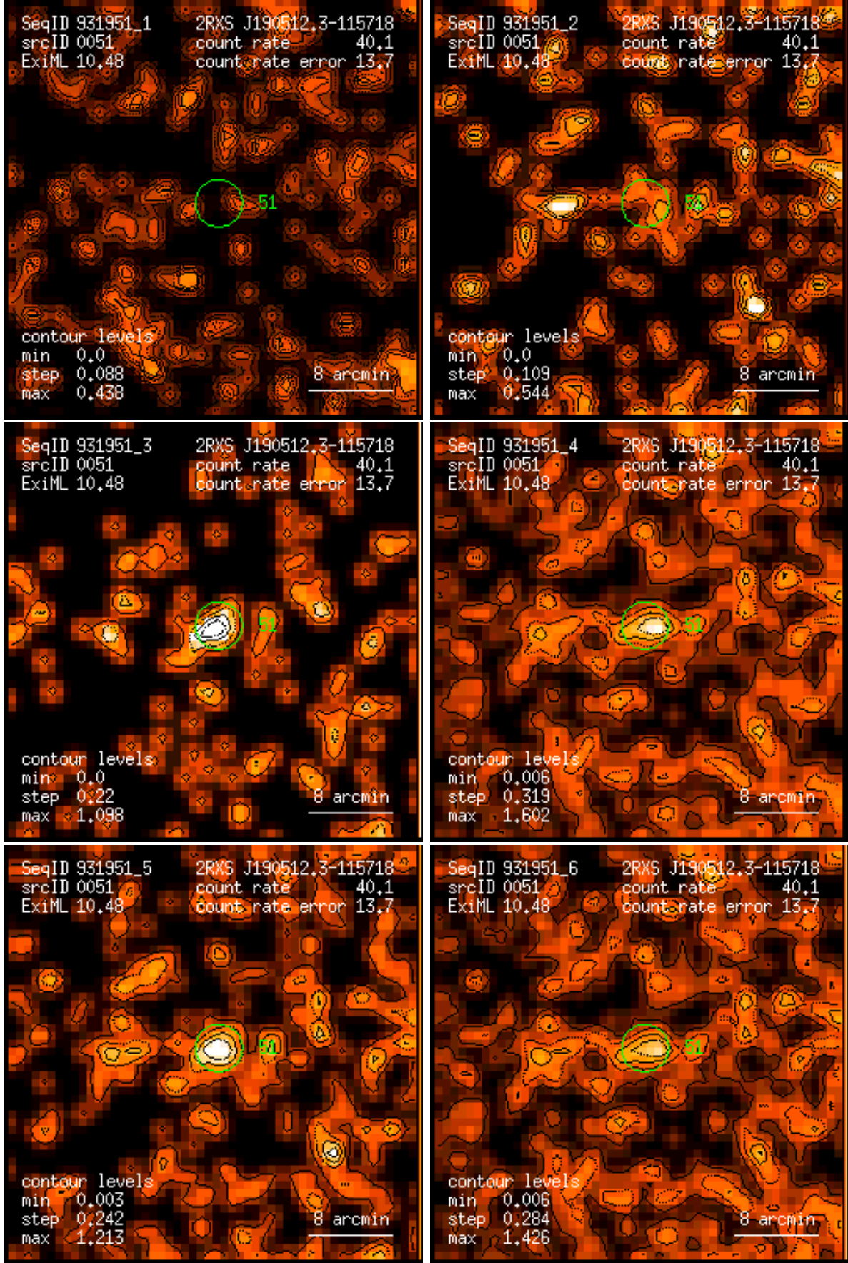
Figure 51: RASS 931951: detection 0051: band rate images, Gaussian filter: (1) PSPC channels 11 – 41, (2) 52 – 90, (3) 91 – 201, (4) 11 – 235, (5) 52 – 201, (6) 11 – 201. Broad band rates in counts/ks. Band rate contour levels in counts/ks/arcmin 2 .
