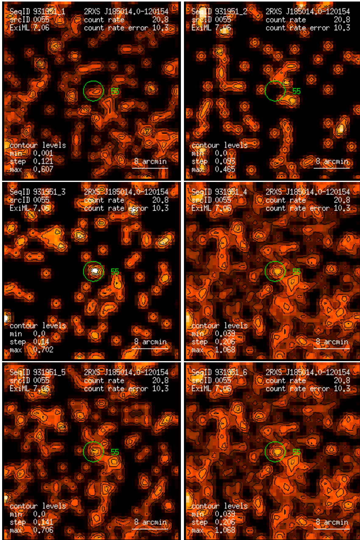
Figure 55: RASS 931951: detection 0055: band rate images, Gaussian filter: (1) PSPC channels 11 – 41, (2) 52 – 90, (3) 91 – 201, (4) 11 – 235, (5) 52 – 201, (6) 11 – 201. Broad band rates in counts/ks. Band rate contour levels in counts/ks/arcmin 2 .
