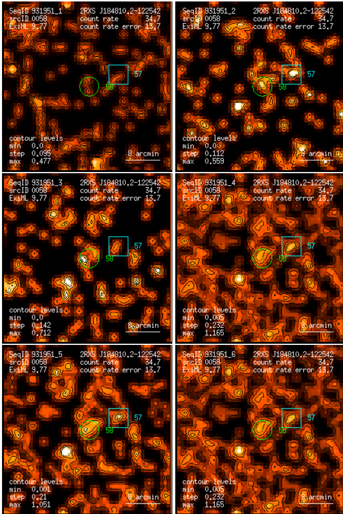
Figure 58: RASS 931951: detection 0058: band rate images, Gaussian filter: (1) PSPC channels 11 – 41, (2) 52 – 90, (3) 91 – 201, (4) 11 – 235, (5) 52 – 201, (6) 11 – 201. Broad band rates in counts/ks. Band rate contour levels in counts/ks/arcmin 2 .
