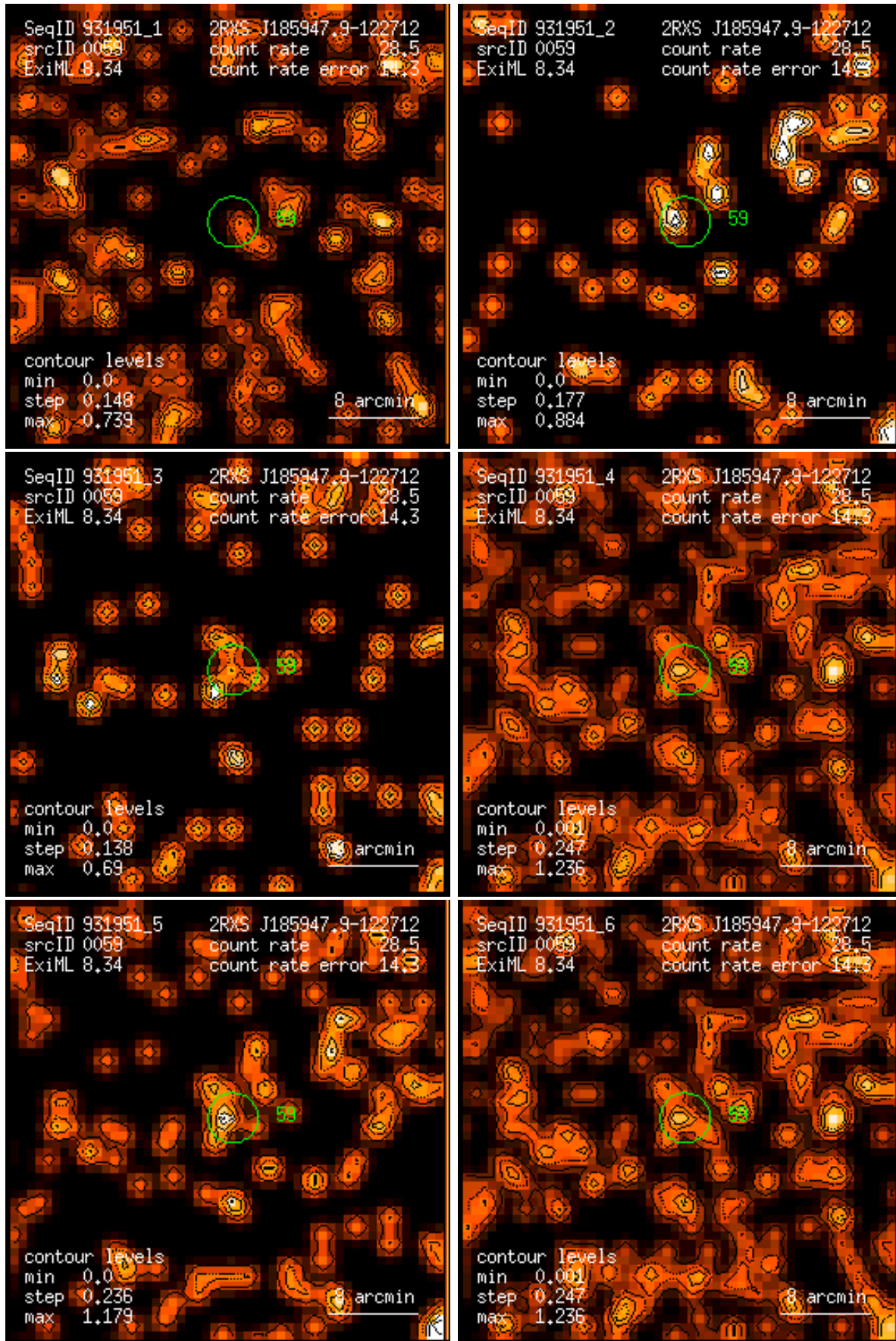
Figure 59: RASS 931951: detection 0059: band rate images, Gaussian filter: (1) PSPC channels 11 – 41, (2) 52 – 90, (3) 91 – 201, (4) 11 – 235, (5) 52 – 201, (6) 11 – 201. Broad band rates in counts/ks. Band rate contour levels in counts/ks/arcmin 2 .
