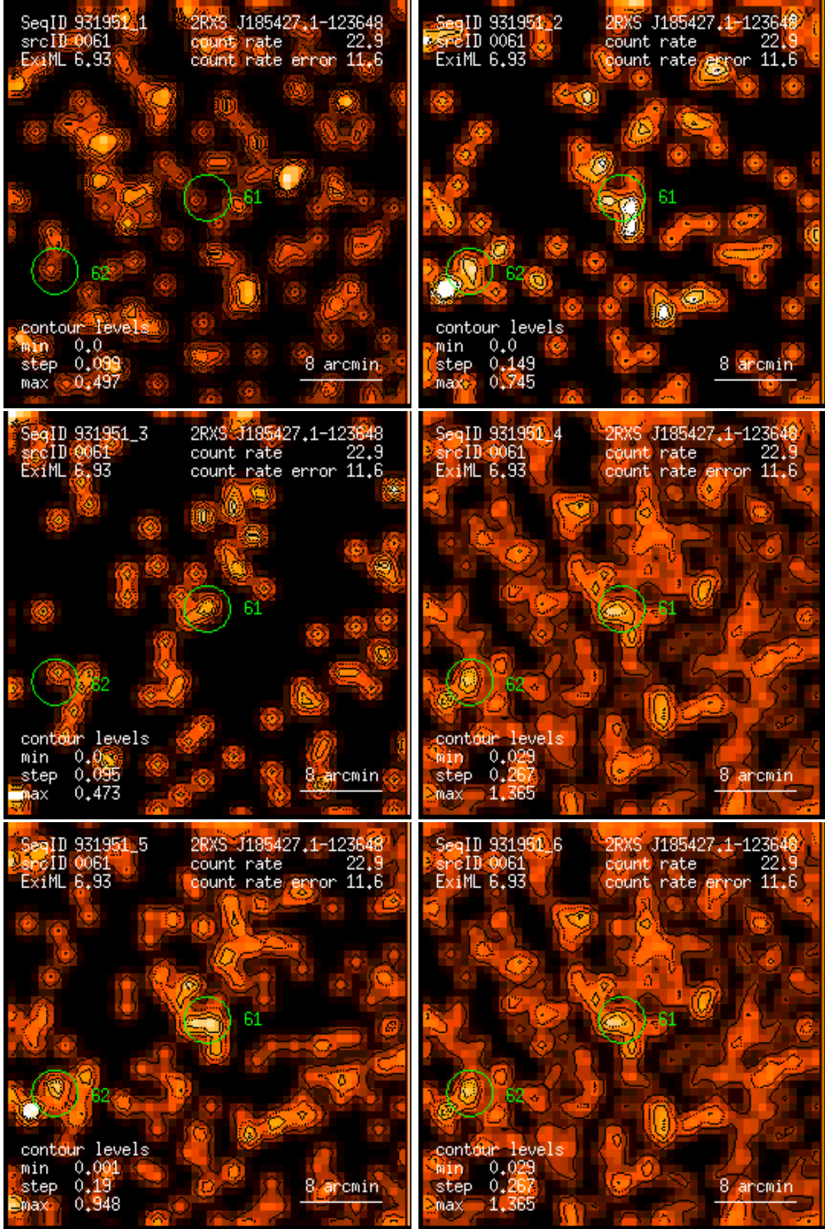
Figure 61: RASS 931951: detection 0061: band rate images, Gaussian filter: (1) PSPC channels 11 – 41, (2) 52 – 90, (3) 91 – 201, (4) 11 – 235, (5) 52 – 201, (6) 11 – 201. Broad band rates in counts/ks. Band rate contour levels in counts/ks/arcmin 2 .
