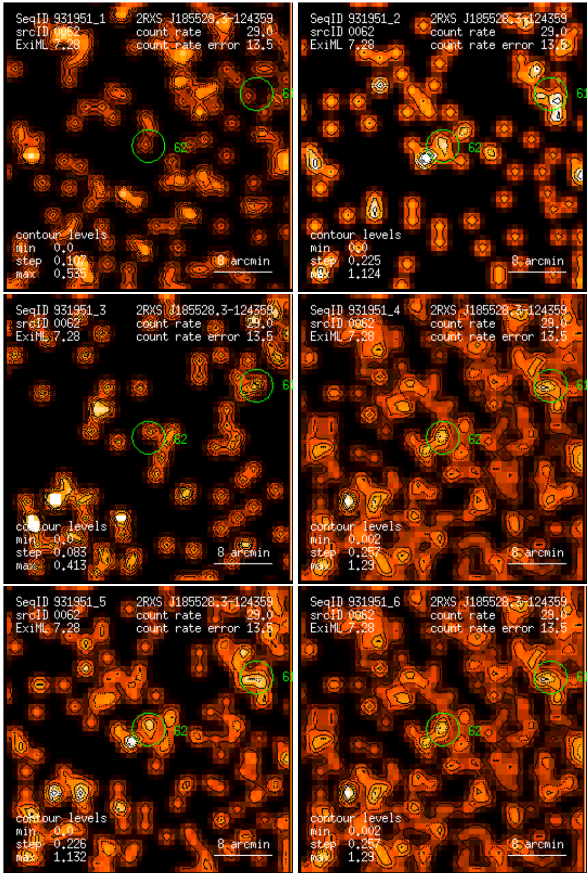
Figure 62: RASS 931951: detection 0062: band rate images, Gaussian filter: (1) PSPC channels 11 – 41, (2) 52 – 90, (3) 91 – 201, (4) 11 – 235, (5) 52 – 201, (6) 11 – 201. Broad band rates in counts/ks. Band rate contour levels in counts/ks/arcmin 2 .
