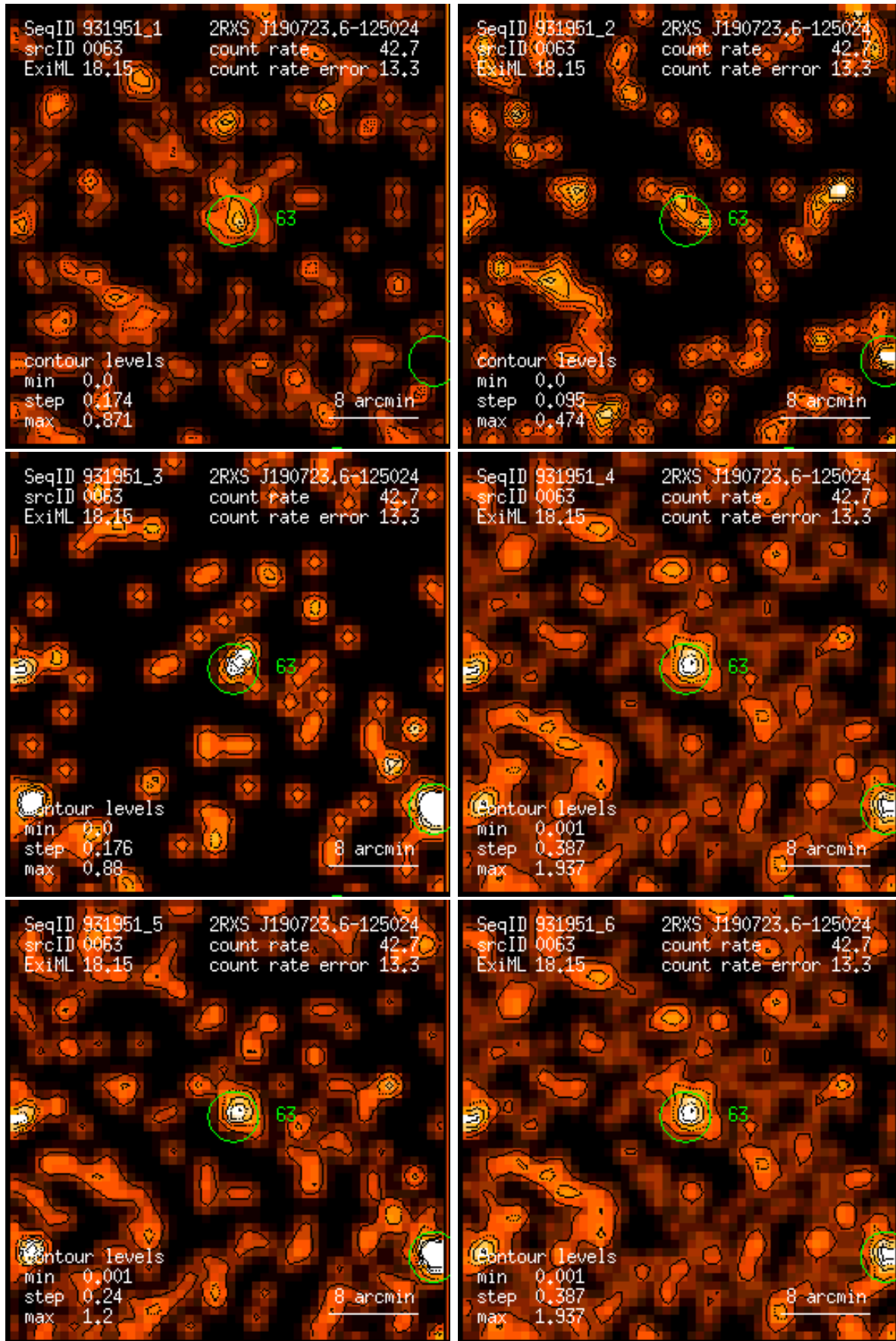
Figure 63: RASS 931951: detection 0063: band rate images, Gaussian filter: (1) PSPC channels 11 – 41, (2) 52 – 90, (3) 91 – 201, (4) 11 – 235, (5) 52 – 201, (6) 11 – 201. Broad band rates in counts/ks. Band rate contour levels in counts/ks/arcmin 2 .
