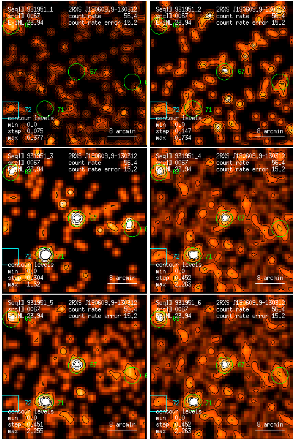
Figure 67: RASS 931951: detection 0067: band rate images, Gaussian filter: (1) PSPC channels 11 – 41, (2) 52 – 90, (3) 91 – 201, (4) 11 – 235, (5) 52 – 201, (6) 11 – 201. Broad band rates in counts/ks. Band rate contour levels in counts/ks/arcmin 2 .
