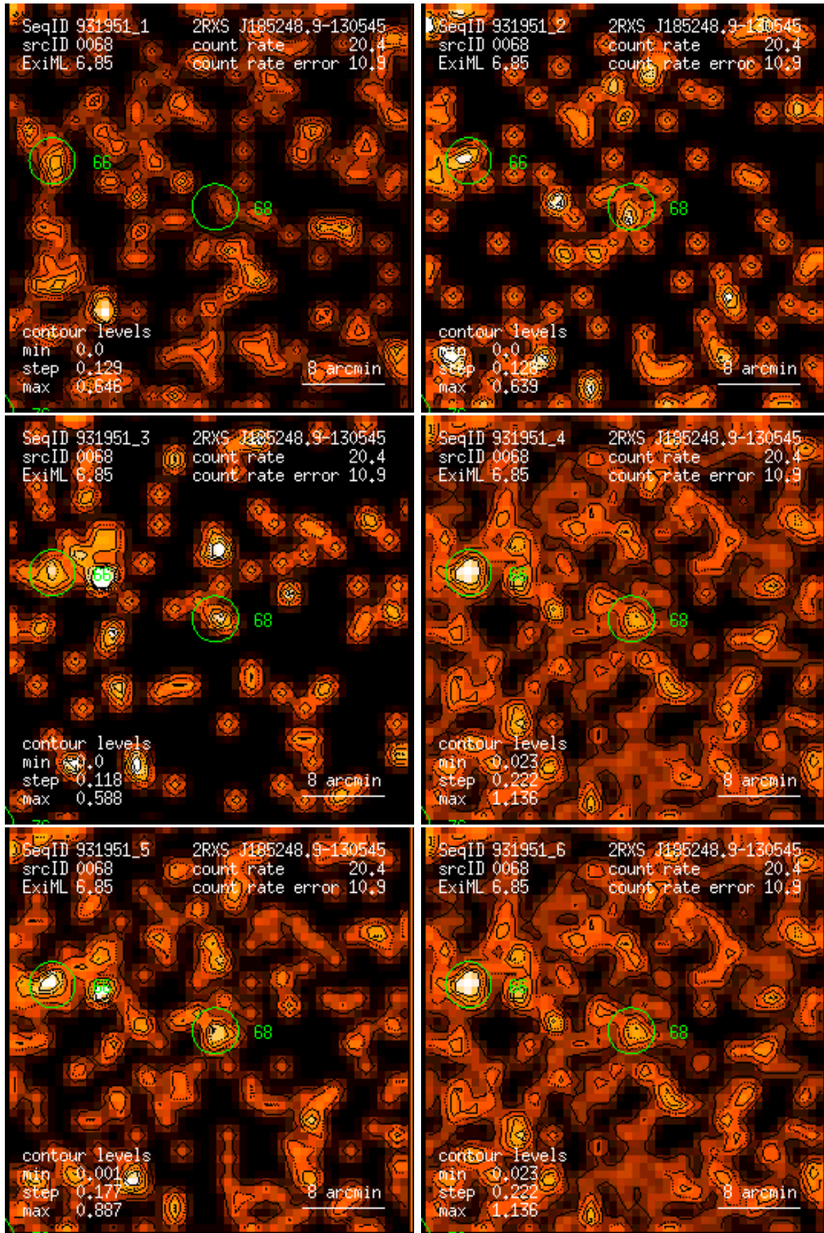
Figure 68: RASS 931951: detection 0068: band rate images, Gaussian filter: (1) PSPC channels 11 – 41, (2) 52 – 90, (3) 91 – 201, (4) 11 – 235, (5) 52 – 201, (6) 11 – 201. Broad band rates in counts/ks. Band rate contour levels in counts/ks/arcmin 2 .
