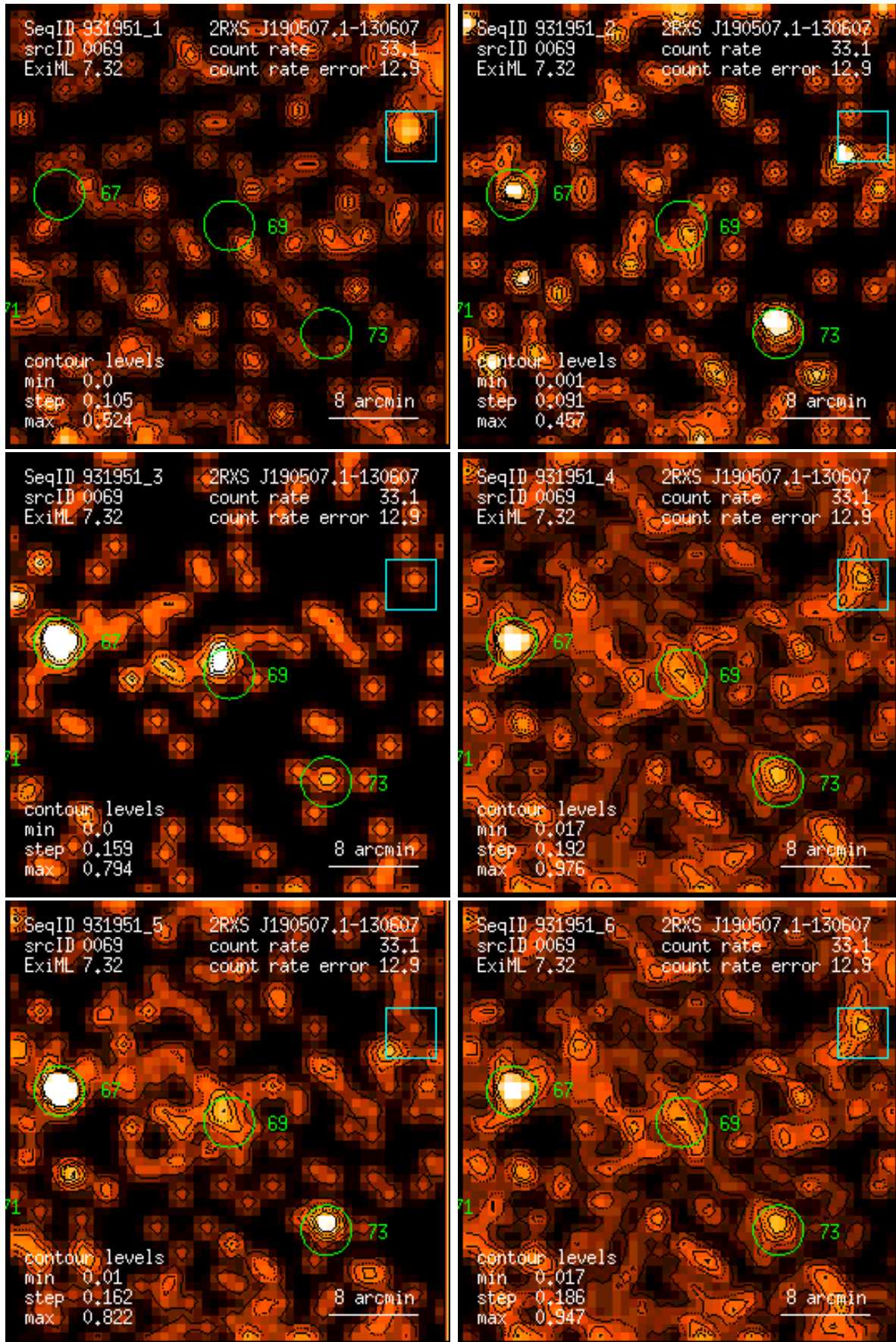
Figure 69: RASS 931951: detection 0069: band rate images, Gaussian filter: (1) PSPC channels 11 – 41, (2) 52 – 90, (3) 91 – 201, (4) 11 – 235, (5) 52 – 201, (6) 11 – 201. Broad band rates in counts/ks. Band rate contour levels in counts/ks/arcmin 2 .
