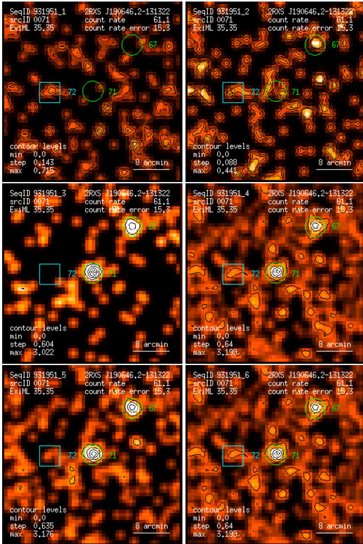
Figure 71: RASS 931951: detection 0071: band rate images, Gaussian filter: (1) PSPC channels 11 – 41, (2) 52 – 90, (3) 91 – 201, (4) 11 – 235, (5) 52 – 201, (6) 11 – 201. Broad band rates in counts/ks. Band rate contour levels in counts/ks/arcmin 2 .
