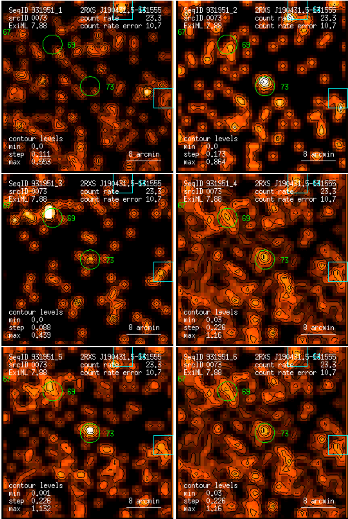
Figure 73: RASS 931951: detection 0073: band rate images, Gaussian filter: (1) PSPC channels 11 – 41, (2) 52 – 90, (3) 91 – 201, (4) 11 – 235, (5) 52 – 201, (6) 11 – 201. Broad band rates in counts/ks. Band rate contour levels in counts/ks/arcmin 2 .
