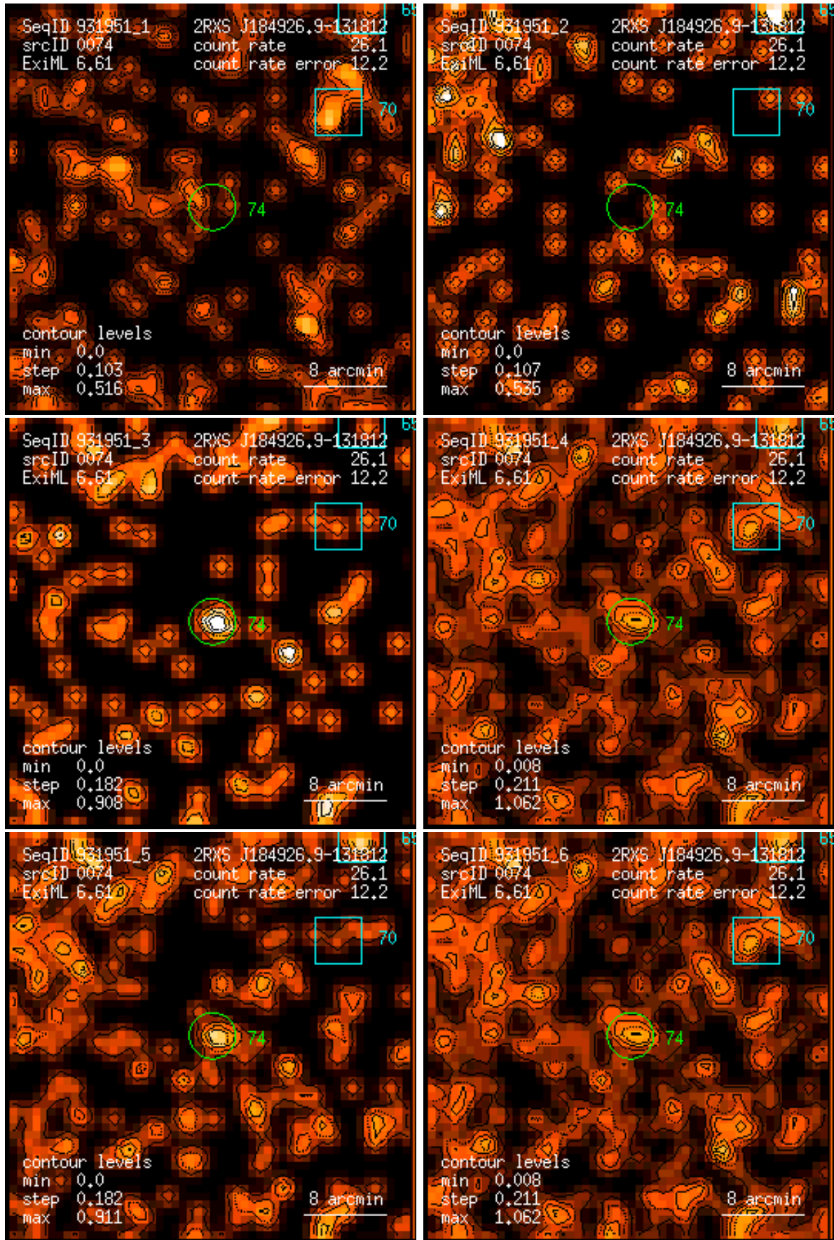
Figure 74: RASS 931951: detection 0074: band rate images, Gaussian filter: (1) PSPC channels 11 – 41, (2) 52 – 90, (3) 91 – 201, (4) 11 – 235, (5) 52 – 201, (6) 11 – 201. Broad band rates in counts/ks. Band rate contour levels in counts/ks/arcmin 2 .
